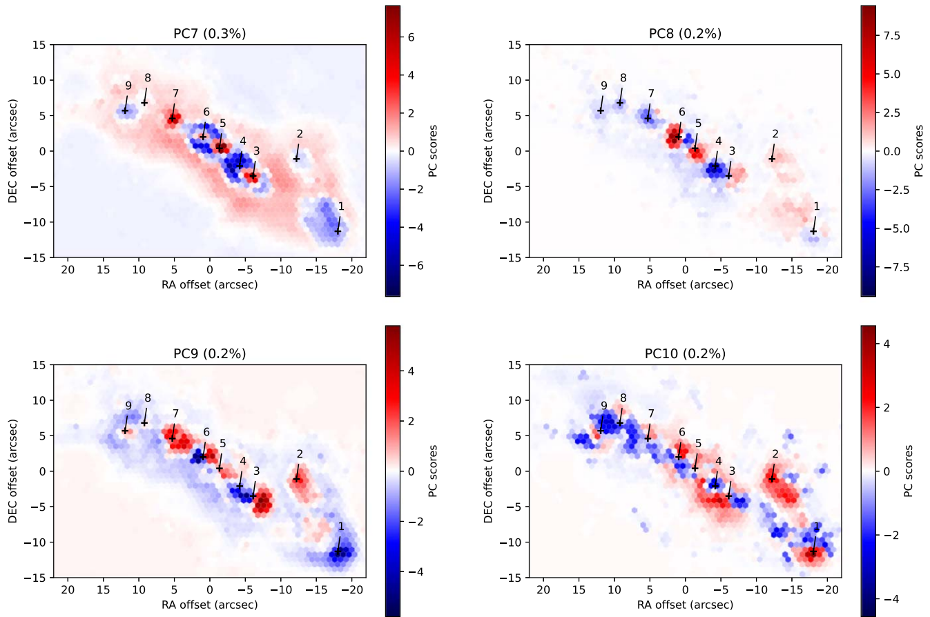
Figure 25. The same as Figure 24, but for PC7–PC10.
