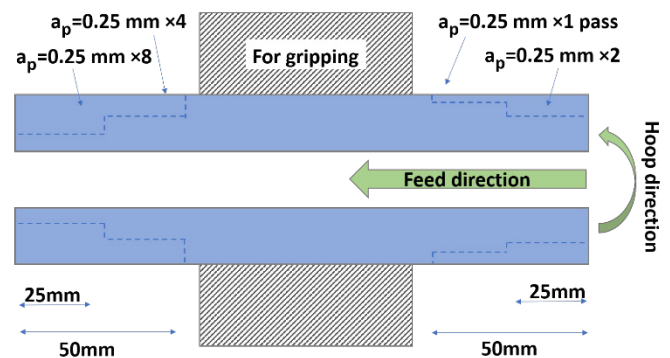
Fig. 1. Schematic illustration of a “stair-profile” cutting strategy for turn-finishing experiments.
