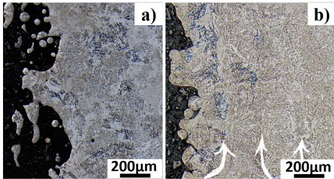
Fig. 3. Cross sections of as-built surfaces without HIP a) no-contour b) three-contours.
