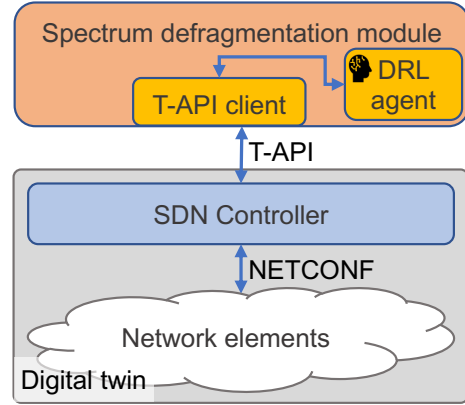
Fig. 2: Demonstrator architecture.
