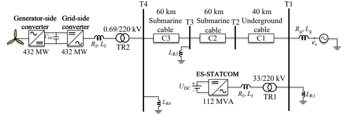
Fig. 2. Simplified model of the considered WPP.
