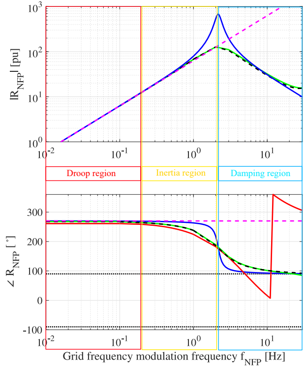
Fig. 12. The NFP plot of an ideal SC (blue curves), a GFM converter (green curves), GFL converter (red curve) and the WPP with a GFM ES-STATCOM (dashed-black curves). The amplitude response of the GFL converter is below the y-axis' lower limit and therefore is omitted from the figure.
