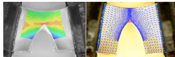
Figure 3: Symmetry-constraint Compact Tension (symconCT) test to explore the fracture properties of aortic wall tissue [9]. Digital Image Correlation (DIC) full-field strain measurements (left) and FEM predictions using a cohesive fracture model (right) are superimposed on the test specimen.
