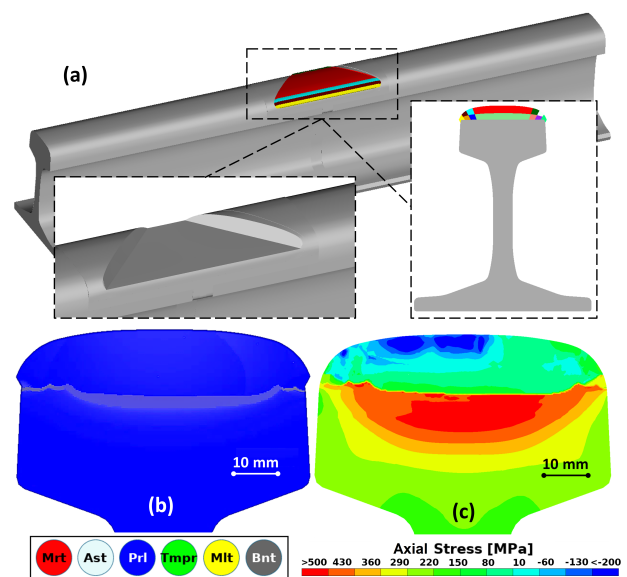
Figure 1: a) FE-model of the rail head with weld passes modelled. b) predicted material phases. c) calculated residual longitudinal residual stress after repair welding and over-rolling operation.
