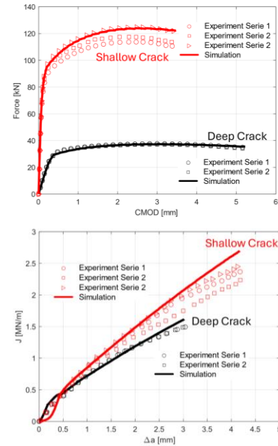
Figure 2: Calibration of SENB with initial deep and shallow crack.
