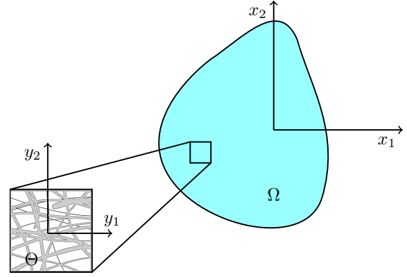
Figure 1: Multiscale spatial domains. The mechanical response at the macroscopic domain \Omega is governed by the response of an X-ray based fibrous unit cell domain \Theta .
