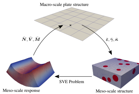
Figure 1: Illustration of computational homogenisation for plates.
