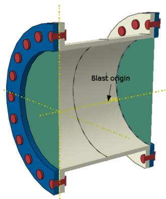
Figure 1: Barrel assembly - Barrel (white), Metal clamps (blue), Composite plates (green), Bolts (red).
