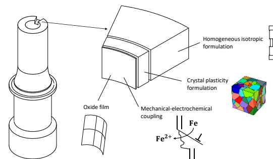
Figure 2: Corrosion fatigue model of metal pipes.
