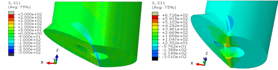
Figure 2: Stress \sigma_{xx} in the piston head for misalignment angles 0.11^\circ (left) and 0.22^\circ (right) at time 6.3 \mu\text{s} .
