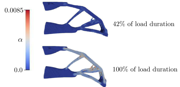
Figure 1: Equivalent plastic strain, after 42 % and 100 % of the maximum load is applied.
