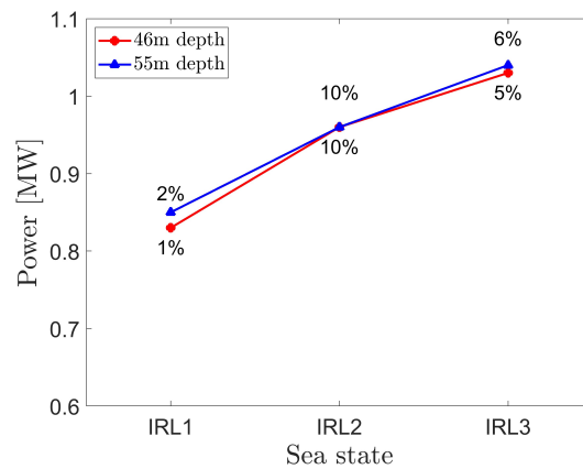
Figure 8. Power output of the 4 \times 4 array layout ( d = 150 m) for the water depths 46 m and 55 m and the irregular sea states IRL 1 to 3. The percentages are the interaction factors indicating the additional power generation due to interaction effects.
