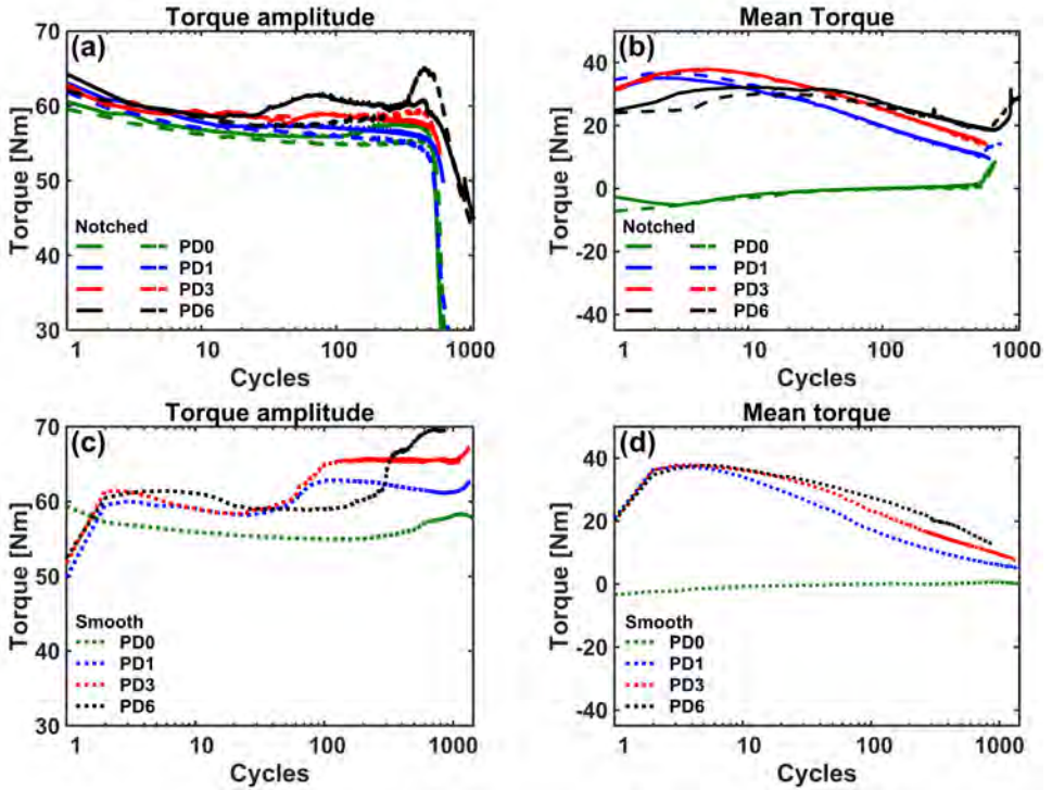
Figure 4.15: Comparison between the torque evolution of notched and smooth test bars for non-proportional loading at \varepsilon_{eq} = 0.6\% : (a) and (b) show the torque amplitude and the mean torque with respect to the number of cycles for notched test bars. (c) and (d) show the torque amplitude and the mean torque with respect to the number of cycles for smooth test bars.
