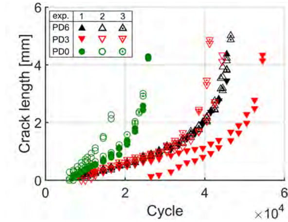
Figure 4.2: Crack propagation measurement from test bars subjected to a load amplitude of 60 % of the offset yield strength.
