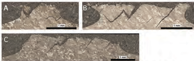
Figure 4.12: Radial view of crack network in a predeformed test bar at different depths from the notch root a) 51 \mu\text{m} b) 234 \mu\text{m} c) 547 \mu\text{m} .
