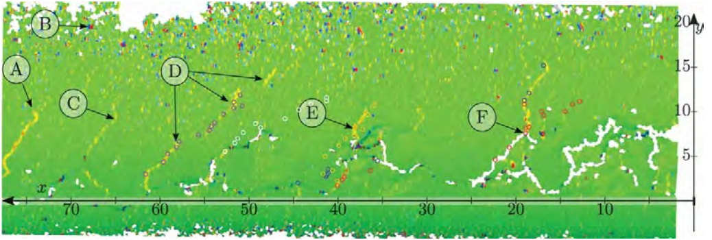
Figure 4.22: Strain field measured by DIC after subjecting the rail section to a bending moment of 15 kNm [43].
