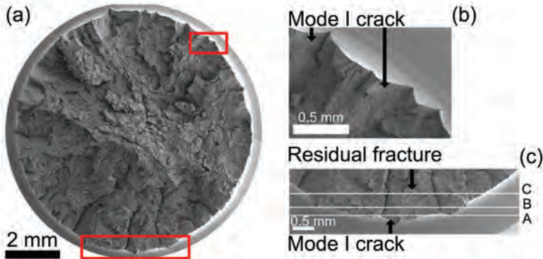
Figure 4.11: Representative fracture surface of predeformed test bars with axial load and shear load along direction of predeformation.
