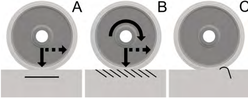
Figure 2.4: Examples of rolling contact fatigue cracks, modified from [14].
