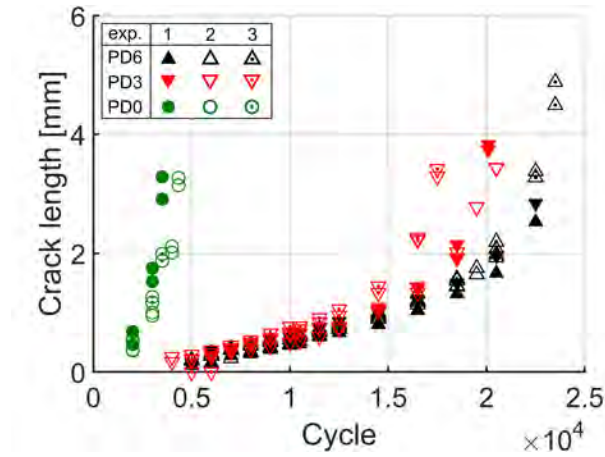
Figure 4.3: Crack propagation measurement from test bars subjected to a load amplitude of 70 % of the offset yield strength.
