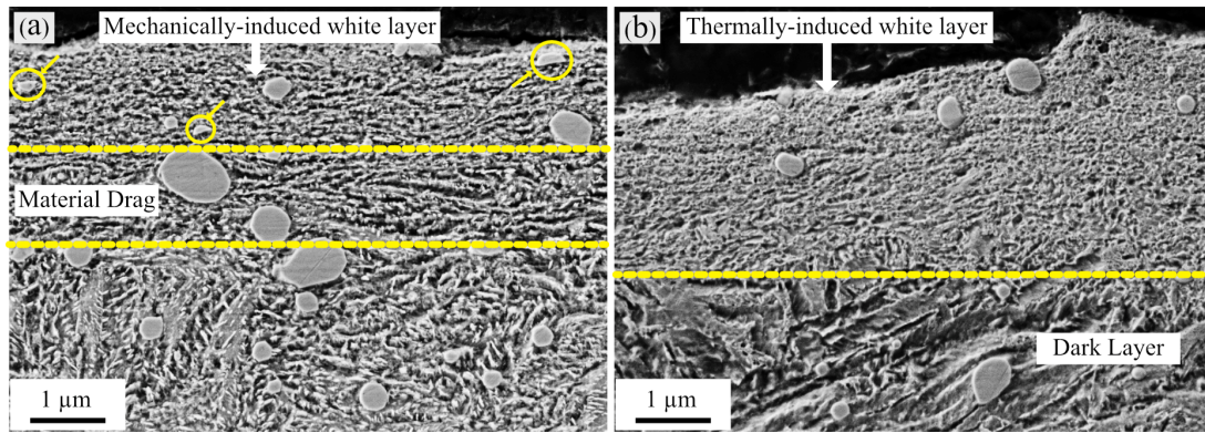
Figure 16: SEM images of the (a) mechanically-induced white layers (M-WL) accompanied with material drag beneath, and (b) thermally-induced white layers (T-WL) with dark layer generated by worn inserts
