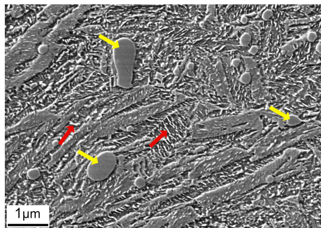
Figure 3: SEM image of the bulk tempered martensite microstructure. Yellow arrows indicate the (\text{Fe, Cr})_3\text{C} carbides in the matrix and red arrows indicate the tempered cementite within the martensite.
