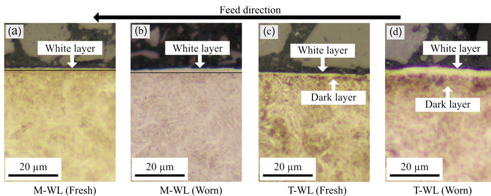
Figure 15: Optical microscopy (OM) images of the mechanically dominant and thermally dominant machined samples with a_p : 0.2 mm, P : 150 bar, \gamma : 35^\circ constant cutting parameters along the feed direction. (a) Fresh insert, f : 0.05 mm/rev, V_c : 60 m/min (M-WL Fresh) (b) VB : \sim 0.2 mm worn insert, f : 0.05 mm/rev, V_c : 60 m/min
