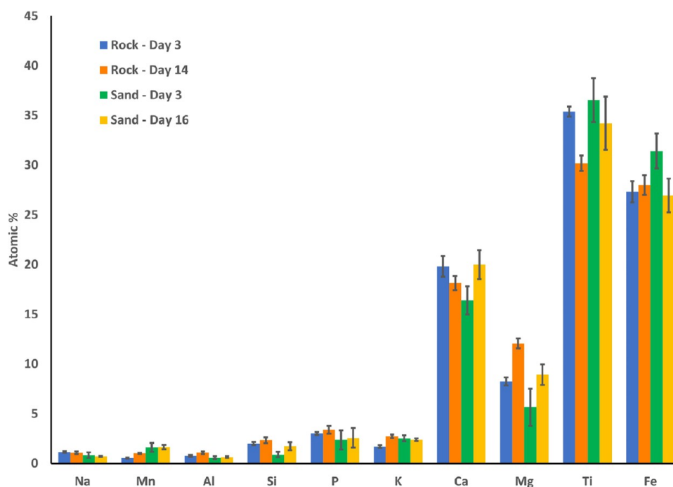
Figure 7. Average elemental composition of bed particle layer on sand ilmenite bed samples taken after 3 and 16 days and rock ilmenite bed samples taken after 3 and 14 days from the FBC process. The values are on a C- and O-free basis, presented in at%, and obtained through SEM-EDS. The error bars show 90% confidence interval for the measured data.
