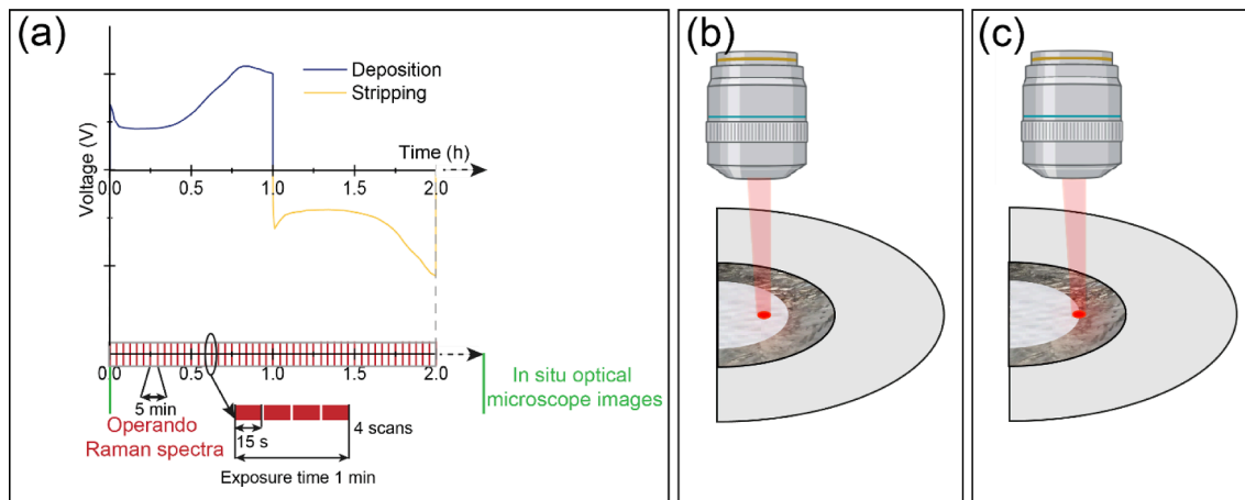
Fig. 1. Schematic representation of the measurement protocol (a) and the sampled areas: ca. 50 \mu\text{m} away from the lithium metal electrolyte interface (b) and between the separator and the working electrode (c).
