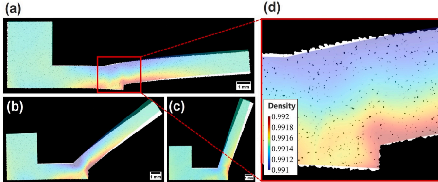
Fig. 15. Comparison of LOM cross-section images with the corresponding virtual cross-section of the sintering simulation results. The different 13 mm angled beams were compared: (a) 15°, (b) 45° and (c) 75°. (d) shows a zoom in the root region of the 15° beam.
