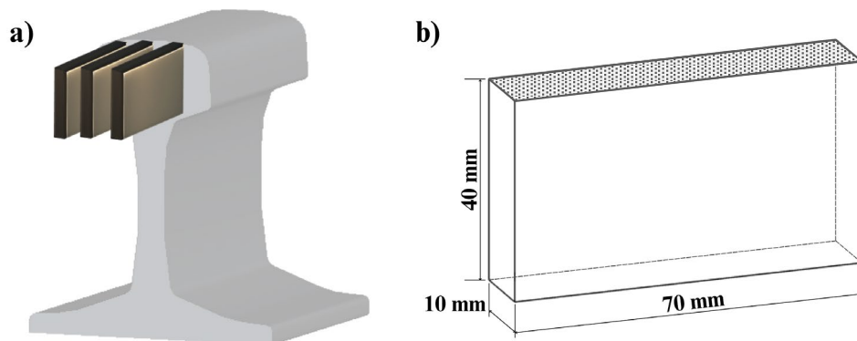
Figure 9: Illustration of the samples for Paper V with (a) showing the position and orientation of the samples taken from the rail head and (b) sample dimensions.
