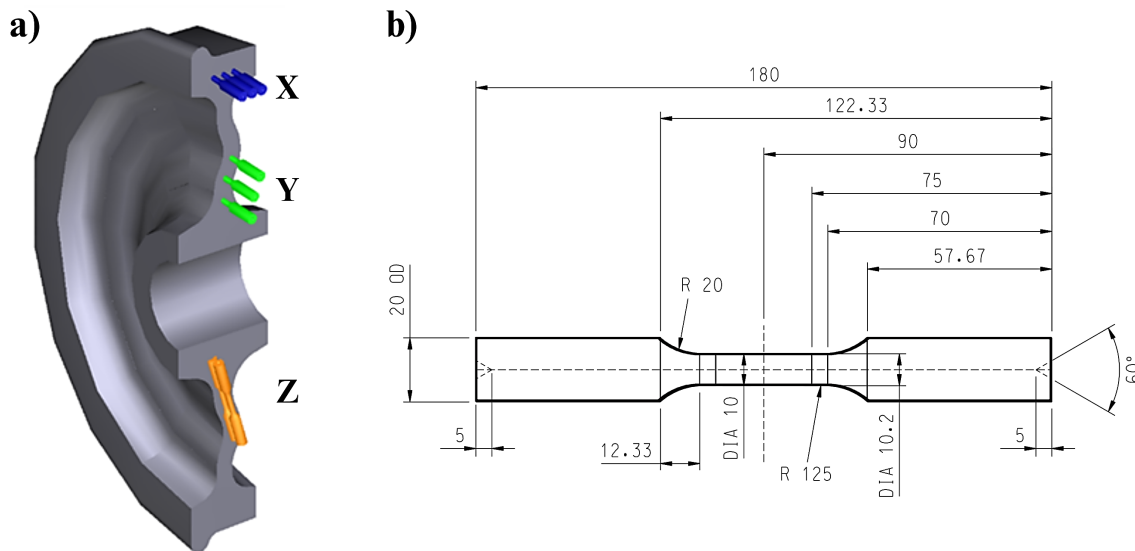
Figure 7: (a) TMF sample locations on virgin ER7T railway wheel. Distinction is made between rim samples (X), circumferential web samples (Y) and radial web samples (Z). (b) Standard test bar geometry as used for Papers I, II and III
