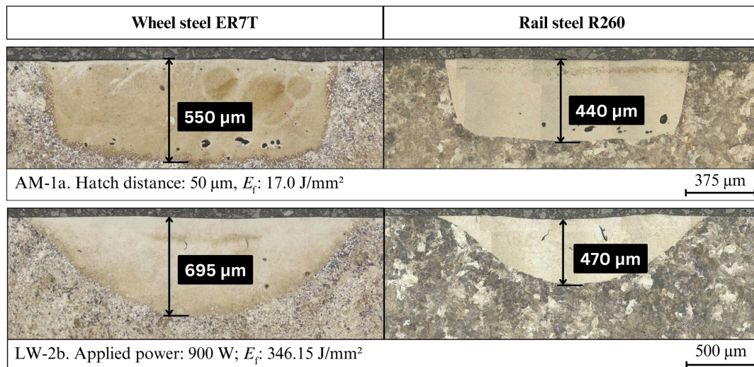
Figure 23: Optical microscopy images of the transformed region created by laser scanning using additive manufacturing equipment (top) and laser welding equipment (bottom). The scan parameters can also be found in Table 3. The same scans were performed on both the near-pearlitic railway wheel steel ER7T (left) and the pearlitic rail steel R260 (right).
