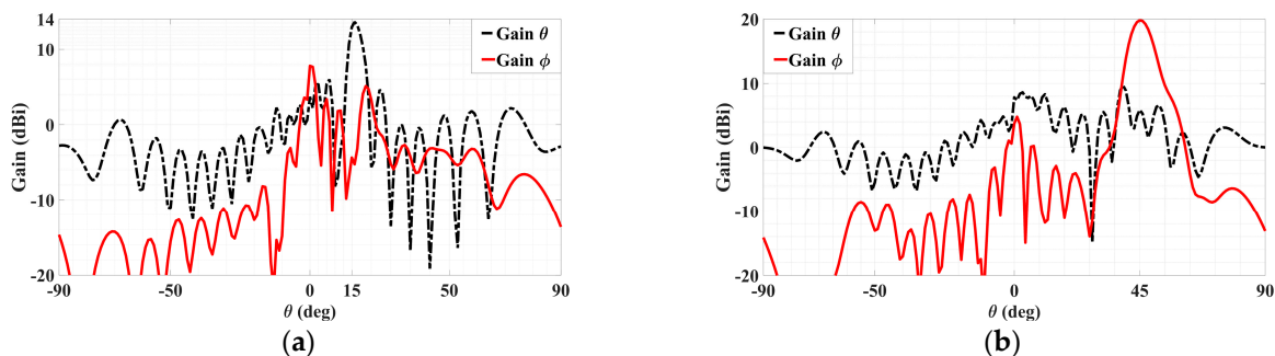
Figure 9. Simulated planar far field patterns for dual-beam, dual-polarized antenna with A^{TM} = 0.333 , A^{TE} = 0.667 , in (a) \phi = \phi_{0m} = 45^\circ plane, showing strong radiation of co-polar theta component but weak cross-polar phi towards \theta_{0m} = 15^\circ , and (b) \phi = \phi_{0e} = 135^\circ plane, showing strong radiation of co-polar phi component but weak cross-polar theta towards \theta_{0e} = 45^\circ . Maximum 20 dBi strength of phi component in is (b) about 20\log_{10}(2) = 6 dB stronger than the 14 dBi strength of theta component in (a).
