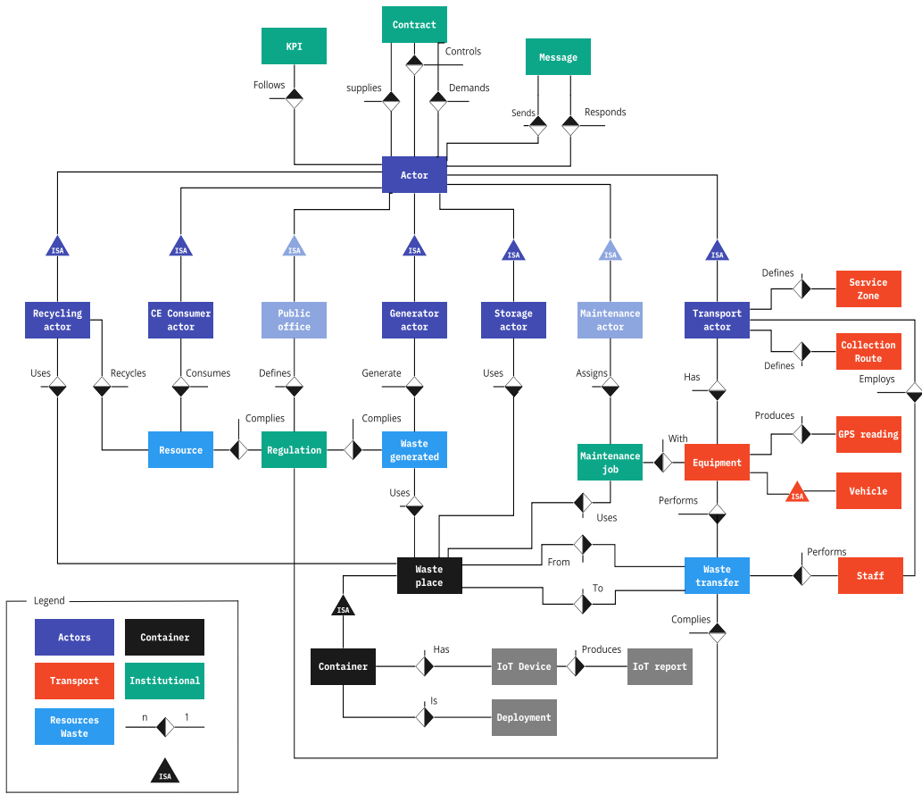
Fig. 4.. Entity Relationship Model (ERM) for waste and resources management - Rein85 notation.
