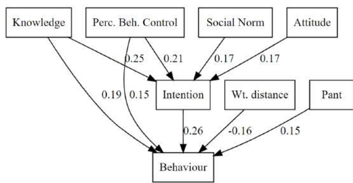
Figure 4.17: Path diagram extracted after Structural Equation Model
