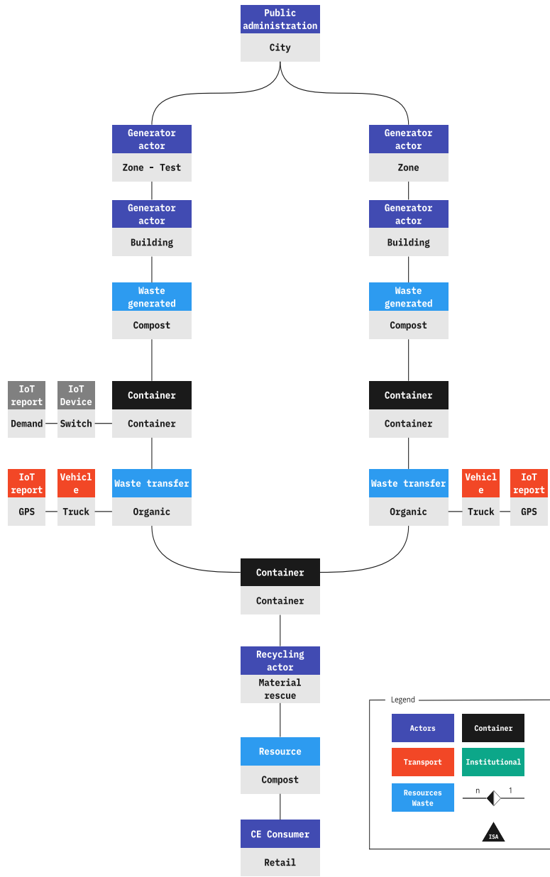
Fig. 7.. Optimization: IoT in waste management operations in Helsingborg.
