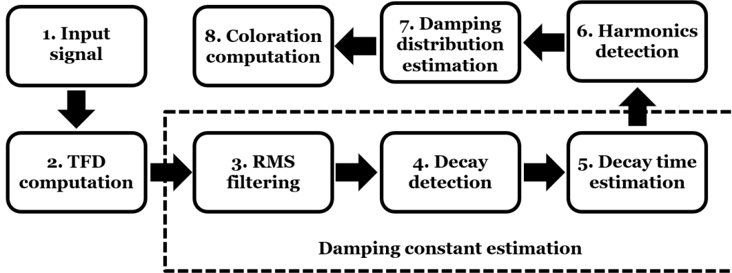
Figure 8.1: The general layout of the coloration detector.
