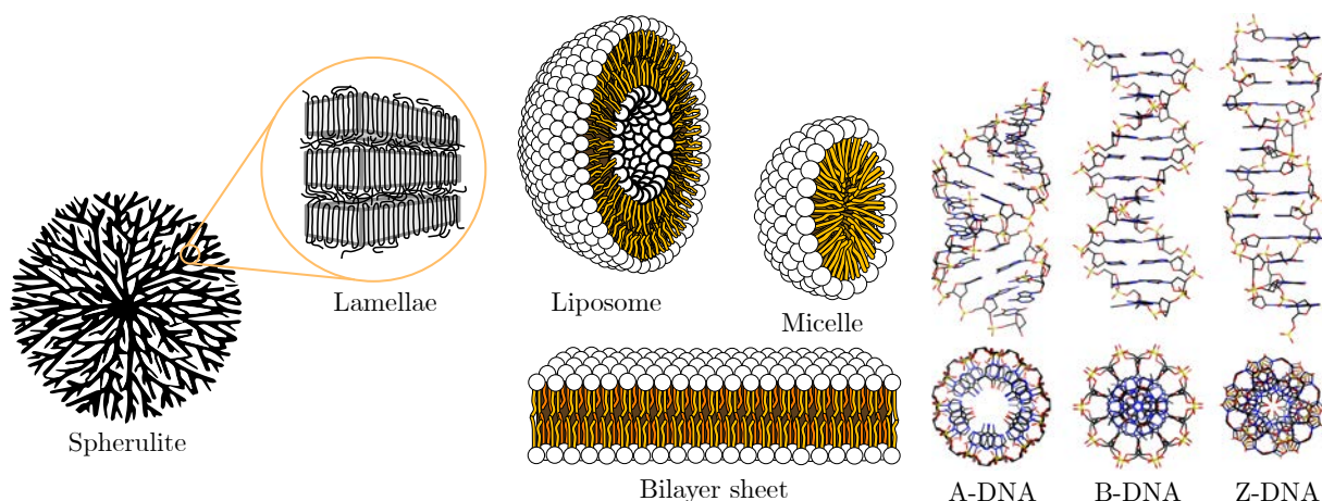
Figure 1.1: Representative structures of soft matter systems showcasing polymers (spherulite and lamellae), phospholipids (liposome, nicelle, and bilayer sheet), and DNA conformations (A-DNA, B-DNA, Z-DNA). These illustrations demonstrate the diverse and flexible nature of soft matter, highlighting their complex behavior under thermal fluctuations and van der Waals interactions. Many of the figures are taken from wikimedia commons.
