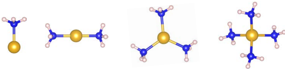
Figure 4.5: Progression of copper-ammonia complexes in the \text{Cu}^+(\text{NH}_3)_x series, showcasing varying numbers of ammonia ligands ( x = 1 to 4 ). Copper is represented by yellow spheres, nitrogen by blue, and hydrogen by white.
