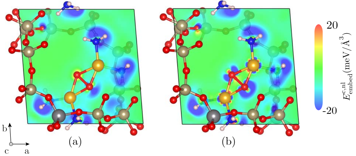
Figure 4.8: Non-local correlation binding energy density \Delta e_c^{\text{nl}}(\mathbf{r}) = E_{\text{embed}}^{\text{c,nl}} (Eq. (3.32)) computed in CX for charged fragments (left) and neutral fragments (right).
