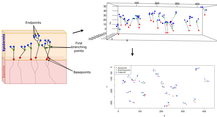
Figure 2.1: An illustration of the ENF data structure (left). An example of the three-dimensional multitype point patterns of the ENF base, branching, and end points (top right) and the corresponding two-dimensional point pattern of the projections (bottom right). The connections between the branching points and the base and end points are also illustrated.
