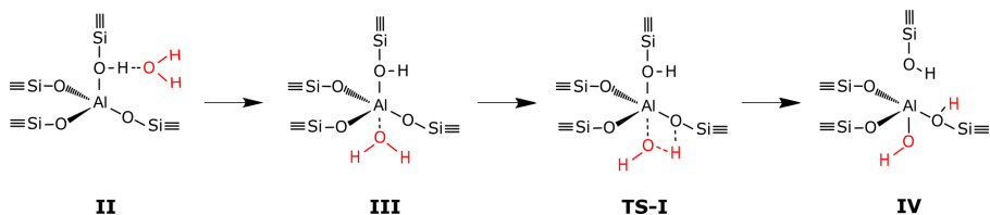
Figure 1.3: Reaction scheme for hydrolysis of the first Al-O bond in H-CHA.
