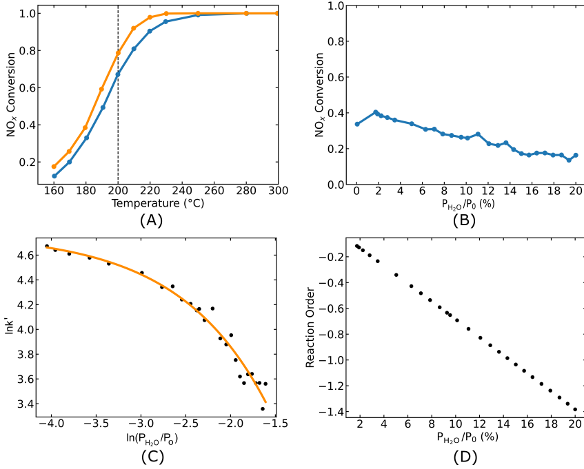
Figure 5.1: NO x conversion over 4% CuO/CHA SAR = 13.4 (A) at different temperatures and (B) at different pressures. (C) Natural logarithm of the rate constant ( \ln(k') ) as a function of the natural logarithm of water partial pressure ( \ln(P_{\text{H}_2\text{O}}/P^0) ). The solid line is a fit to the experimental data. (D) Shows the reaction order in H 2 O as a function of the partial pressure of H 2 O. Reaction conditions (A): 10% O 2 , 500 ppm NO, 600 ppm NH 3 , 5% H 2 O in wet condition. Reaction conditions (B), (C), (D): 200 °C, 10% O 2 , 500 ppm NO, and 600 ppm NH 3 .
