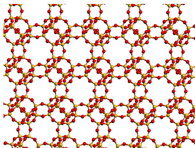
Figure 1.2: Ball and stick model of the CHA structure. Atomic color code: aluminum (purple), silicon (yellow), and oxygen (red).
