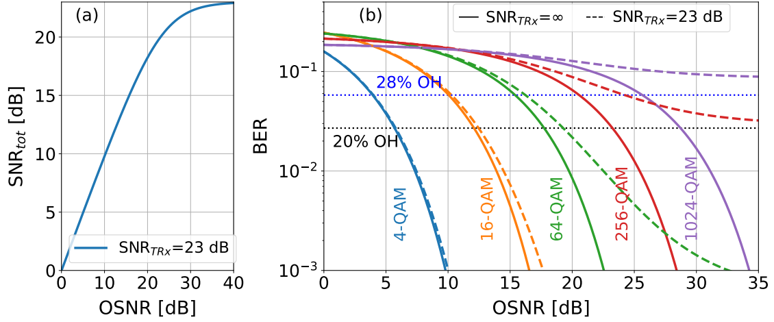
Figure 2.10: Given a fixed SNR_{Tx} = 23 dB, (a) the simulated SNR and (b) BER performance, versus OSNR for various QAM formats.
