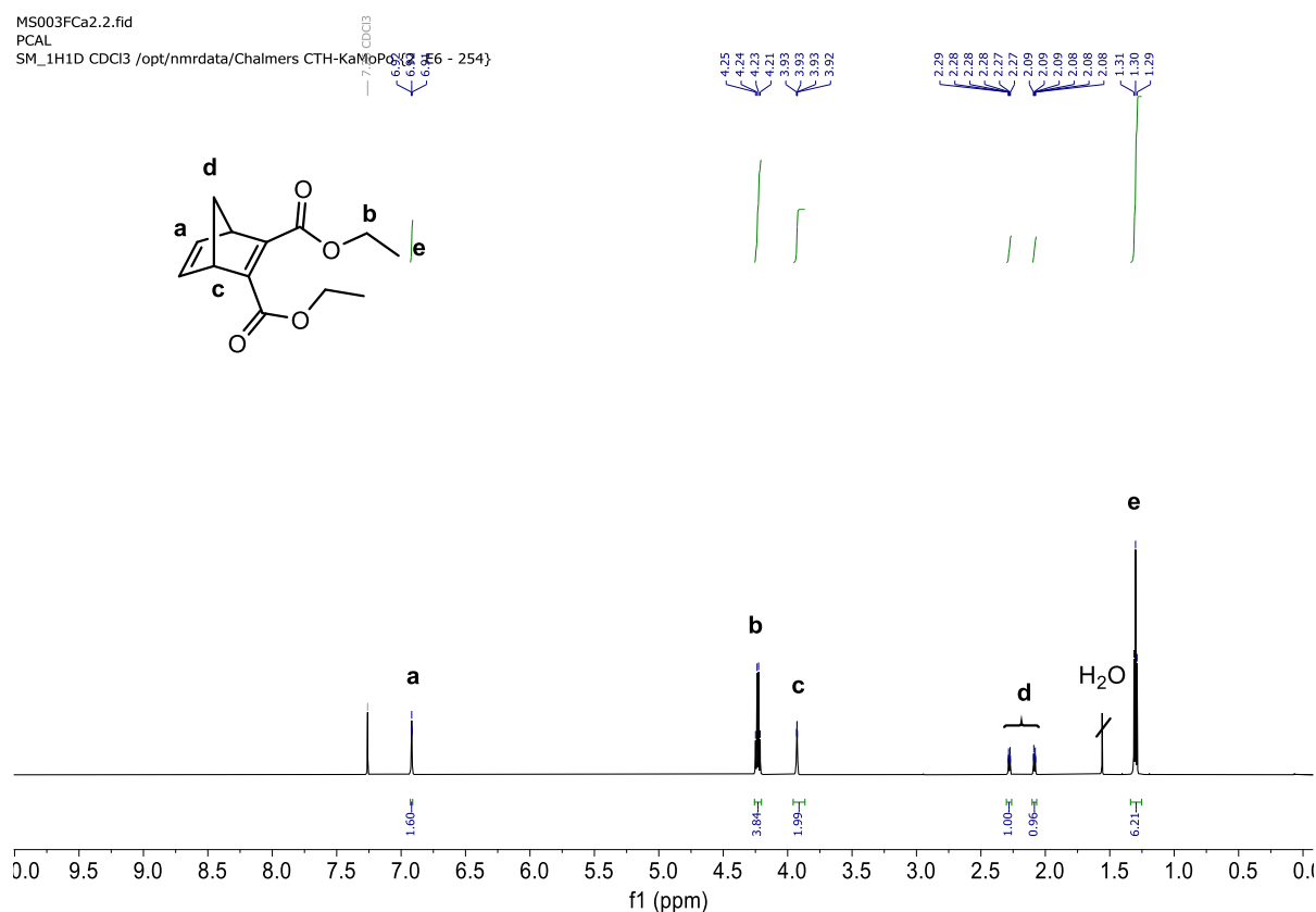
Figure S1. 1 H-NMR spectrum of ( 1a ) in CDCl 3 at 298K.
