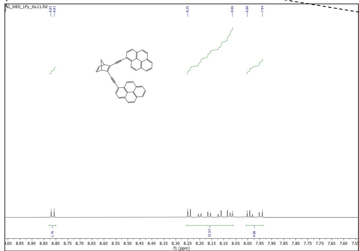
Figure S2: 1 H-NMR spectrum of NBD-1Py.
