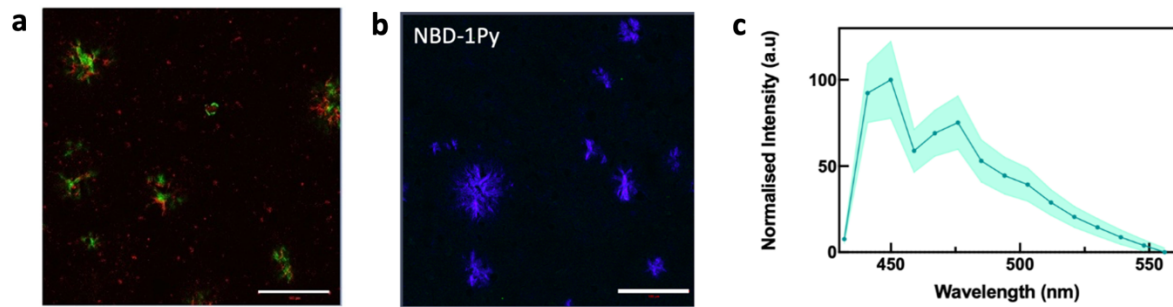
Figure S34: a) Confocal image of Aβ plaques in cortex brain sections of Tg-APP Swe mouse model (21 months, female). Green is NBD-1Py, red is 6E10 anti amyloidβ antibody, white bar = 100 μm; b). Confocal hyperspectral image of Aβ plaques in cortex brain sections of a TgSwe mouse model (21 months, female) obtained with NBD-1Py as a fluorescent stain. White bar = 100 μm. c) In situ measured emission spectra of NBD-1Py when staining the plaques. The mean intensity values over the whole plaques area were extracted, and the average of 3 plaques together with the (green band) is shown.
