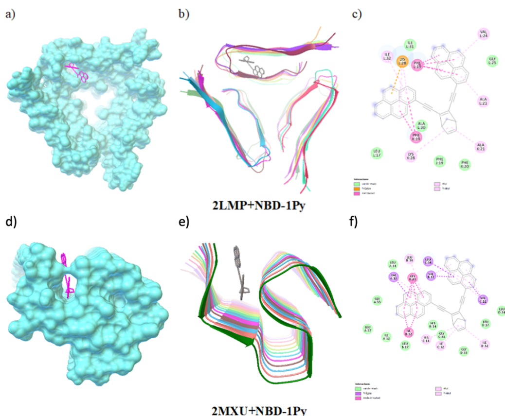
Figure S30: a) to c) Binding modes for NBD-1Py with with the A \beta 1–40 (PDB ID: 2LMP) amyloid plaque, and d) to f) for NBD-1Py with the A \beta 1–42 (PDB ID: 2MXU) amyloid plaque. a) 3D image of the NBD-1Py-2LMP complex (surface of the receptor in light-blue and ligand in magenta). b) 3D image of the NBD-1Py-2LMP complex (receptor represented as ribbons and ligand with carbons in gray. Hydrogens are omitted for clarity). c) 2D-diagram of the interactions of NBD-1Py with 2LMP.
