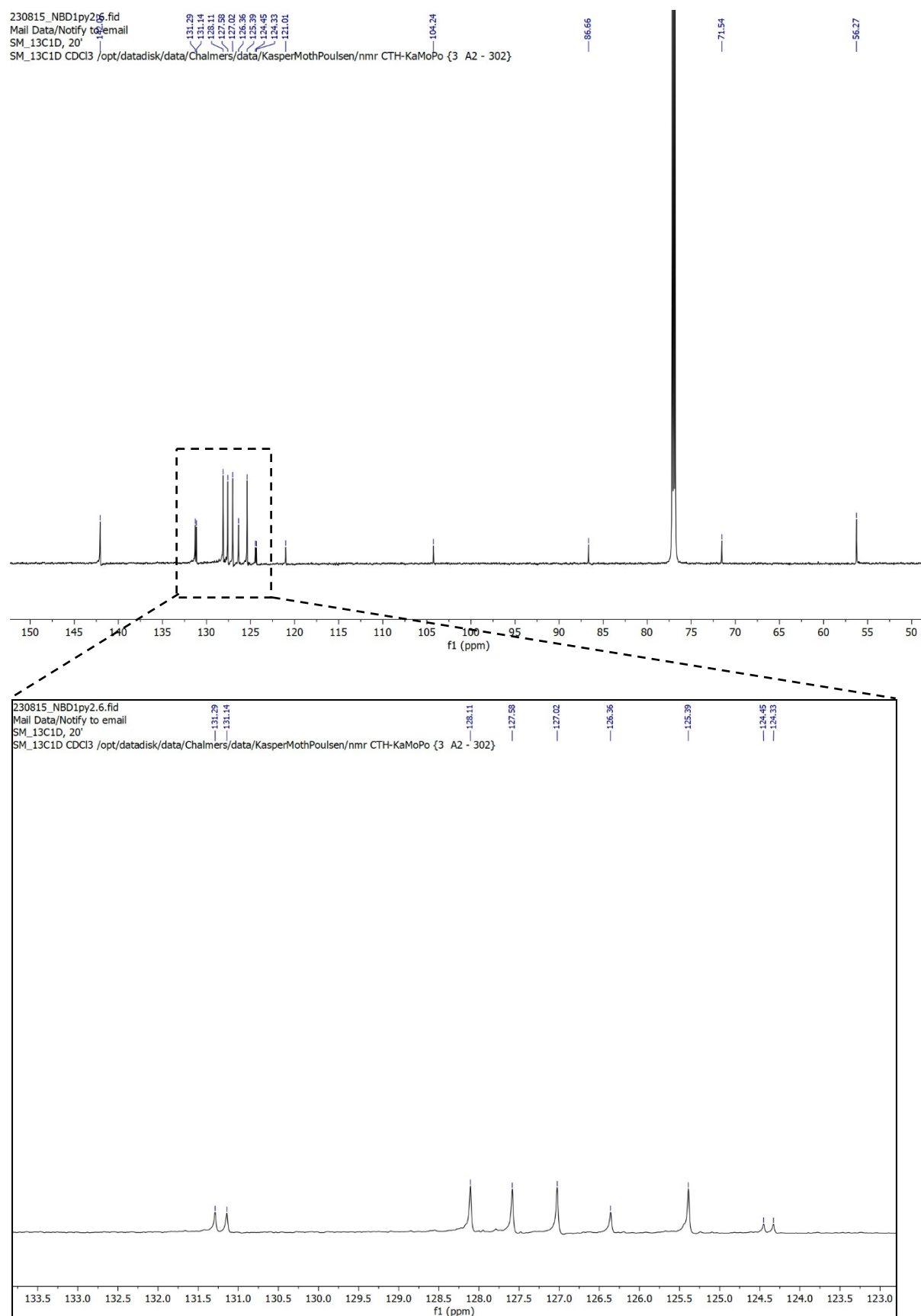
Figure S4: 13 C-NMR spectrum of NBD-2Py.
