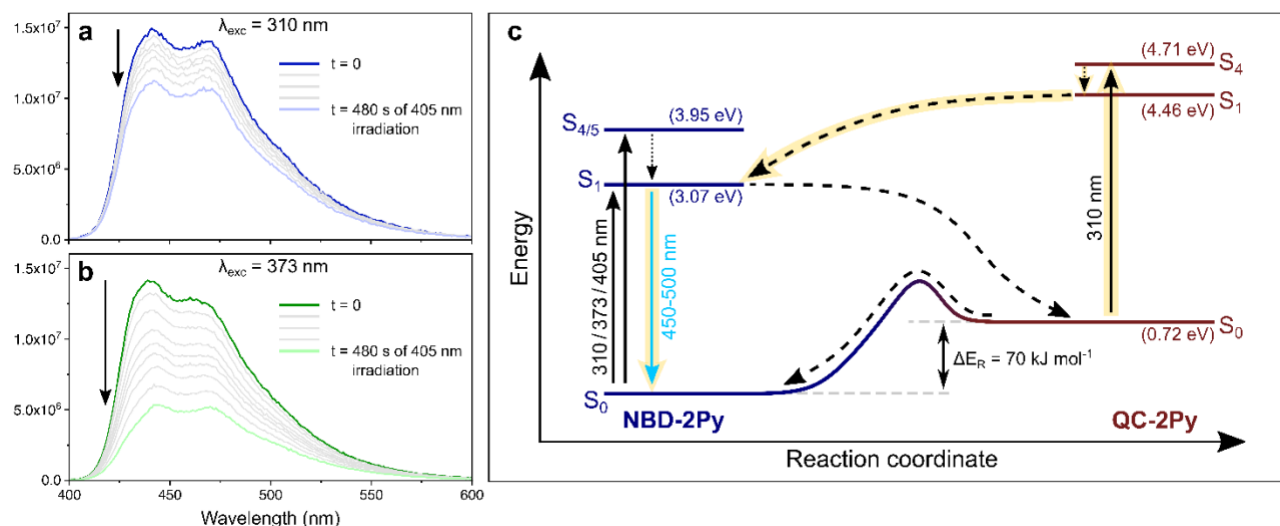
Figure 3: Steady state emission of NBD-2Py measured directly after different times (0–480 s) of exposure to 405 nm continuous-wave irradiation at 0°C. (a) \lambda_{exc} = 310 nm. (b) \lambda_{exc} = 373 nm. (c) Proposed reaction pathways in NBD-2Py. Highlighted in yellow is the suggested reaction pathway of photoinitiated back conversion from QC-2Py to NBD-2Py.
