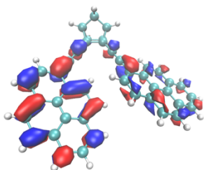
Figure S16: Hole orbital involved in the S 0 -S 1 transition in QC-1Py.
