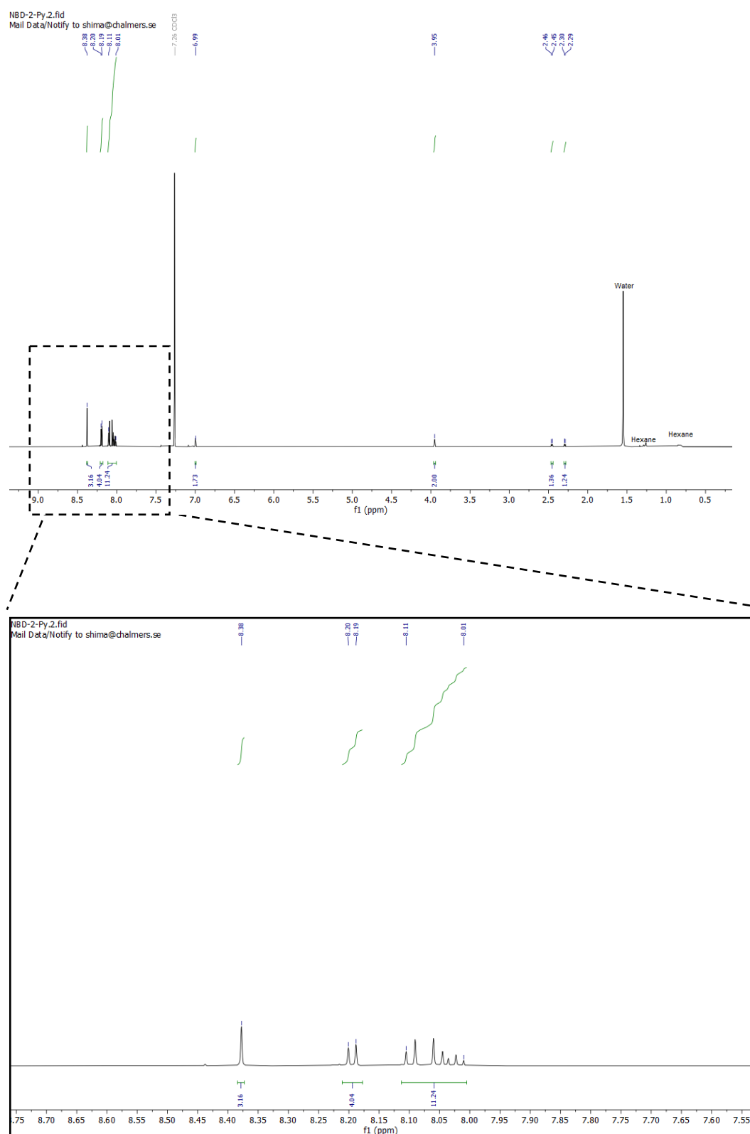
Figure S1: ^1\text{H} -NMR spectrum of NBD-2Py.
