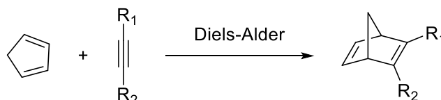
Figure 4. Synthesis of donor/acceptor norbornadienes via Diels-Alder reaction. R_1 and R_2 are acceptor and donor groups.
