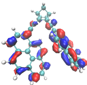
Figure S14: Hole orbital involved in the S 0 -S 3 transition in NBD-1Py.
