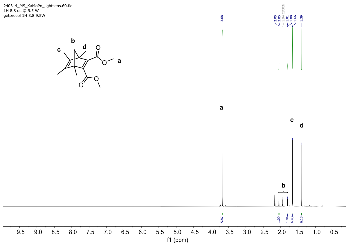
Figure S7. ^1\text{H} -NMR spectrum of ( 7a ) in \text{CD}_3\text{CN} at 298K.
