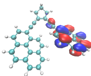
Figure S13: Particle orbital involved in the S 0 -S 3 transition in NBD-1 Py.
