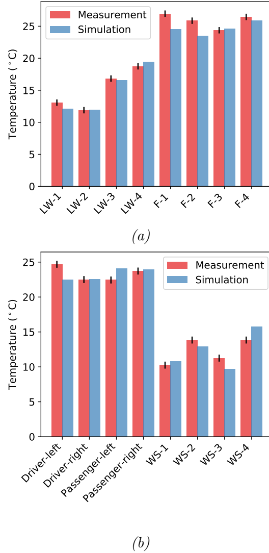
Figure 3.18: Comparison of the thermocouples' temperatures from the numerical simulation and experiment. The uncertainty of the experiments was considered to be the probe's accuracy. (a) Left window and floor thermocouples; (b) Head-level air temperatures and front windshield thermocouples.
