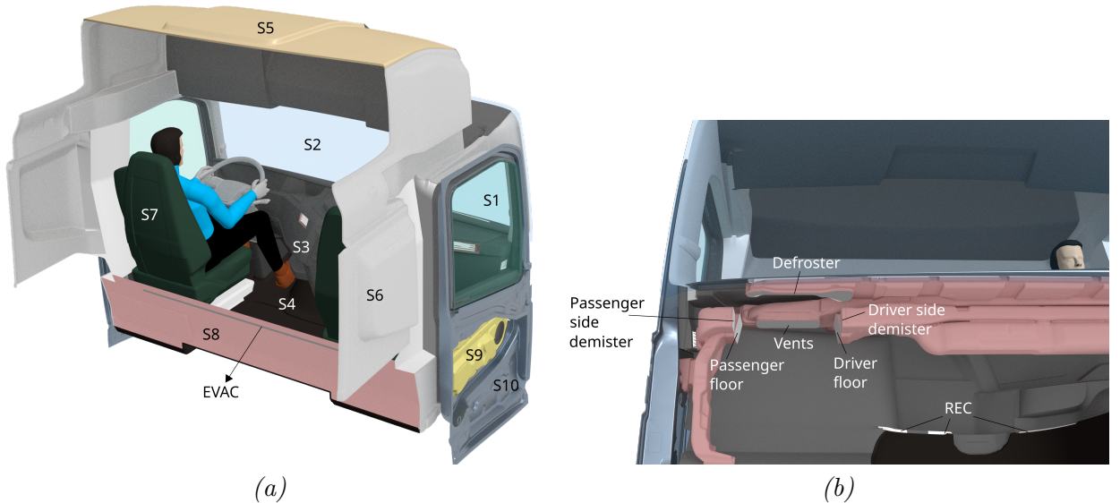
Figure 3.15: (a) Truck cabin with all the interior solids (S1-S10) colored based on the corresponding material property from Table A.2, along with the evacuation outlet (EVAC); (b) Inlets in the cabin and the recirculation outlet (REC).
