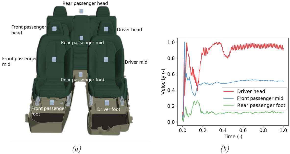
Figure 3.3: (a) The location of nine monitor volumes used in the simulation; (b) Normalized velocity vs time in three monitor volumes. The values were normalized to the maximum instantaneous driver head velocity and the heat-up time.
