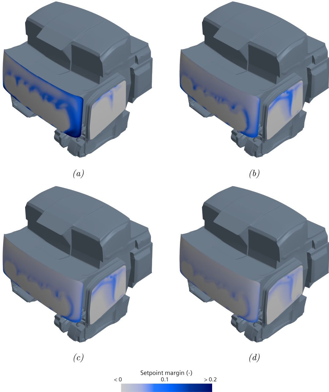
Figure D.4: Region of possible window fogging with varying normalized setpoint margins at different driving speeds (a) 0 km/h; (b) 30 km/h; (c) 60 km/h; (d) 90 km/h.
