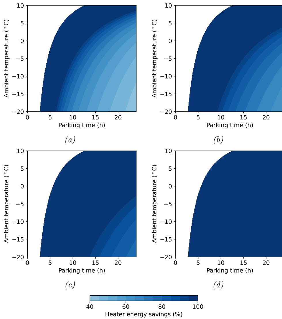
Figure 4.10: Heater energy savings of the encapsulated configurations relative to the baseline, with varying thermal resistances (a) 0.47 \text{ m}^2\text{K/W} ; (b) 0.94 \text{ m}^2\text{K/W} ; (c) 1.72 \text{ m}^2\text{K/W} ; and (d) 3.76 \text{ m}^2\text{K/W} .
