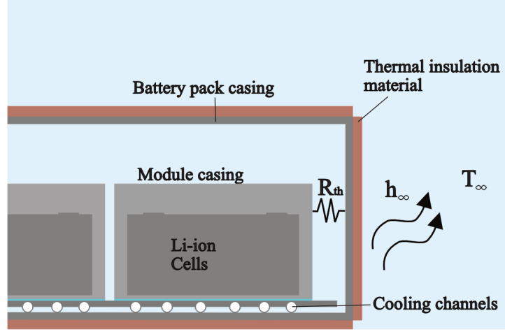
Figure 4.6: Thermal encapsulation of the battery pack.
