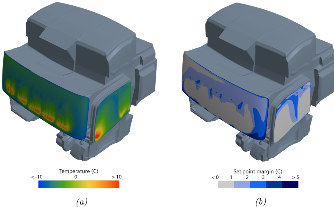
Figure D.1: (a) Temperature distribution on the window for the reference case at -10^\circ\text{C} , 70% RH, and 90 km/h, at the end of 30 minutes. (b) Region of possible fogging with varying setpoint margins.
