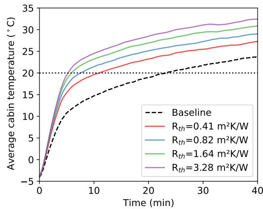
Figure 3.9: Effect of varying magnitudes of insulation resistance on the average cabin temperature vs time.
