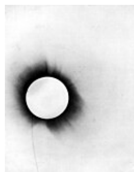
Figure 1.1: Observations of light deflection in 1919. 1
