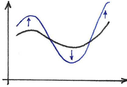
Figure 4.3: Mutations in the team game alters the strategy of the “resident” population and introduces a new “mutant” distribution.
