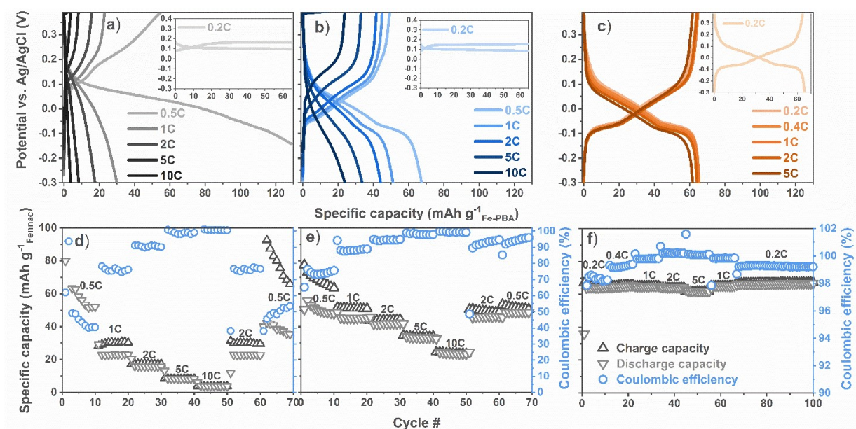
Figure 28. Fennac electrode rate capability tests with a,d) 1.0 m \text{Na}_2\text{SO}_{4(\text{aq})} , b,e) 1.9 m \text{Na}_2\text{SO}_{4(\text{aq})} , and c,f) the Hybrid electrolytes.
