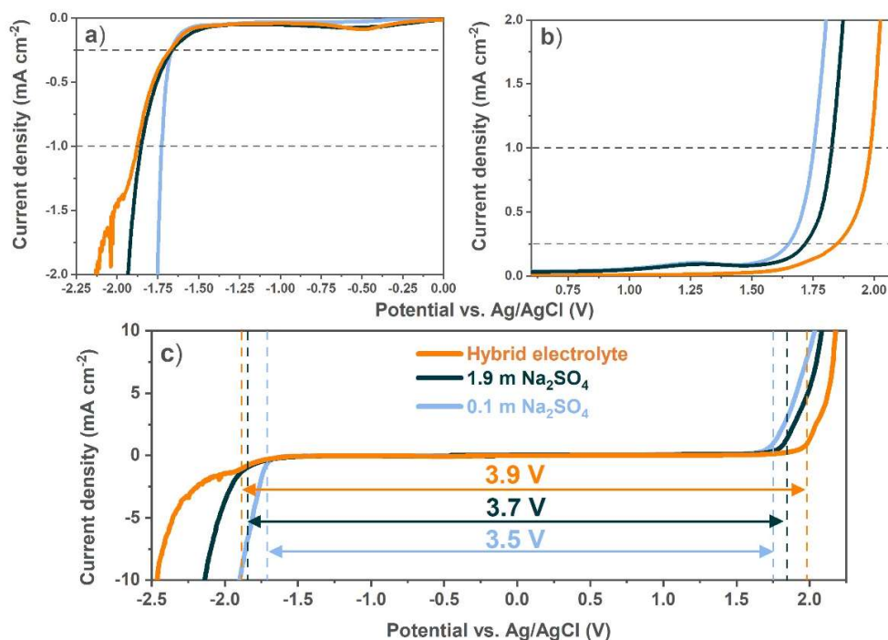
Figure 21. ESW of the aqueous electrolytes measured by LSV. A zoom-in of a) the reduction and b) the oxidation and c) a depiction of the full window. Dashed lines to mark the stability limit. [I].
