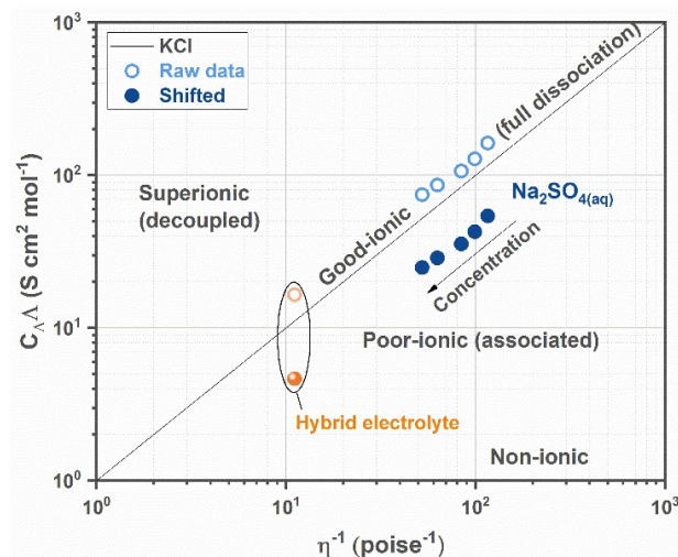
Figure 24. Walden plot of the aqueous electrolytes at 30°C. [I].
