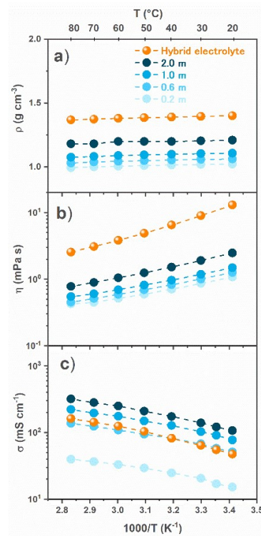
Figure 23. Arrhenius plots of the: a) density, b) viscosity, and c) ionic conductivity for the Na 2 SO 4 -based aqueous electrolytes. Dashed lines to guide the eye only. [I].
