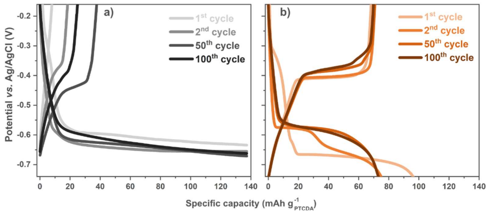
Figure 32. GC charge and discharge curves of PTCDA at 0.2C using a) the 1 m \text{Na}_2\text{SO}_4(\text{aq}) and b) the Hybrid electrolytes. [I].
