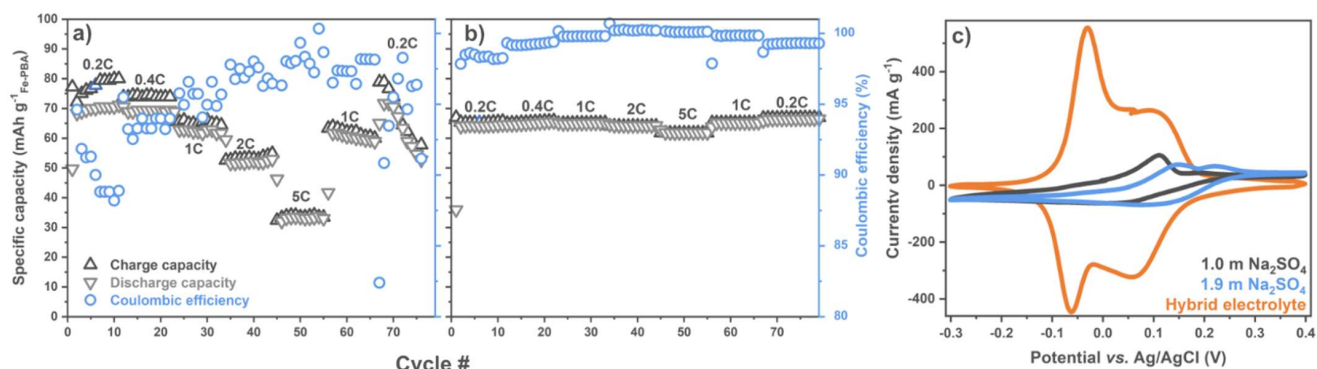
Figure 27. Fe-PBA electrode rate capability tests with a) glassy carbon and b) AC CE with the hybrid electrolyte between 0.4 and -0.3 V vs. Ag/AgCl. c) Fe-PBA voltammograms at 0.2 mV s -1 .
