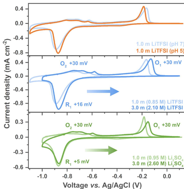
Figure 50. 1 st CV cycle of PTCDA with different a) pH, b) [\text{LiTFSI}_{(\text{aq})}] and c) [\text{Li}_2\text{SO}_{4(\text{aq})}] .
