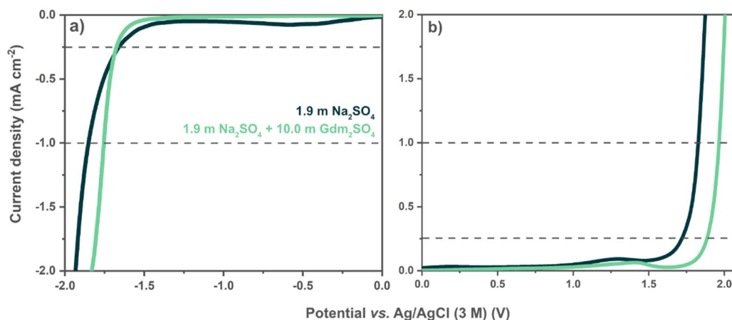
Figure 18. ESW of the aqueous electrolytes measured by LSV. A zoom-in of a) the reduction and b) the oxidation. Dashed lines mark the two stability limits.
