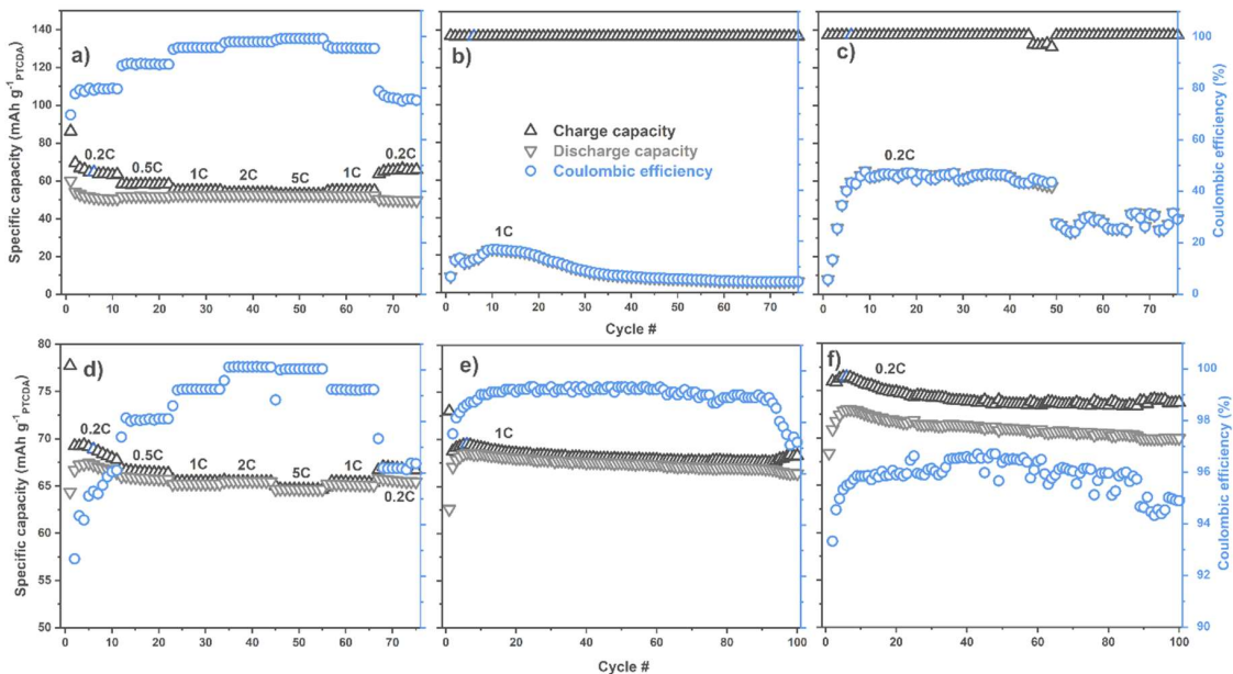
Figure 33. PTCDA electrode a,d) rate capability test and b,c,e,f) GC with a-c) 1 m \text{Na}_2\text{SO}_4(\text{aq}) and d-f) the Hybrid electrolyte. Note the right and left y-axis scale differences between a-c and d-f. [I].
