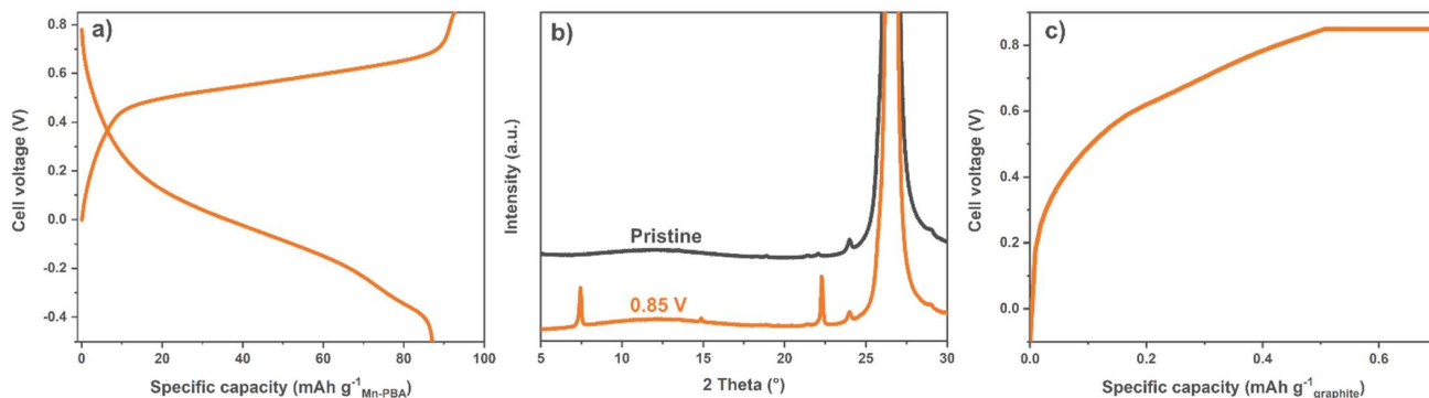
Figure 44. a) Typical charge/discharge curves for the Mn-PBA ex situ characterizations using a two electrode AC||Mn-PBA pseudo half-cell. b) X-ray diffractograms of pristine and oxidized graphite current collectors and c) the corresponding voltage profile (right). [IV]
