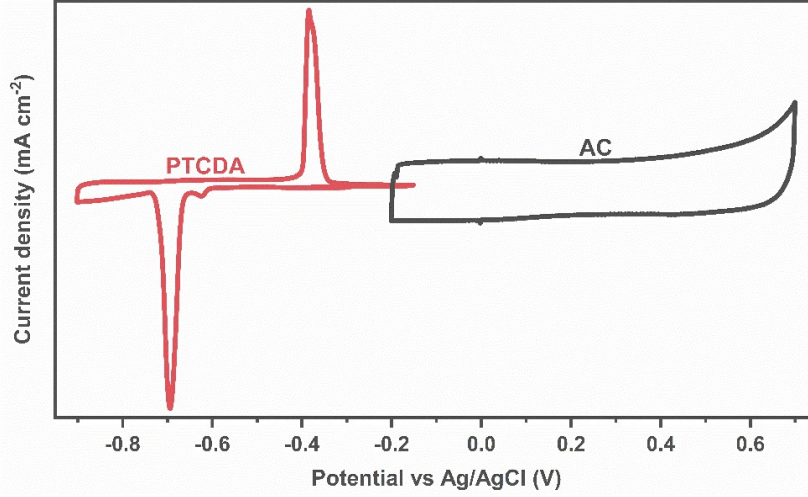
Figure 14. Cyclic voltammogram.
