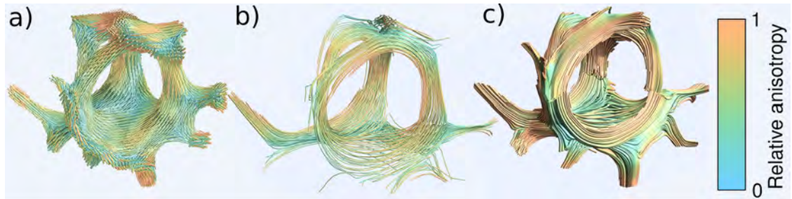
Figure 6.3: a) Cylinder glyph render showing orientation in trabecular bone. b) Streamline render. c) Streamline render after restricting orientations to one hemisphere, by restricting strict positivity of the orientation vector component orthogonal to the large loop.
