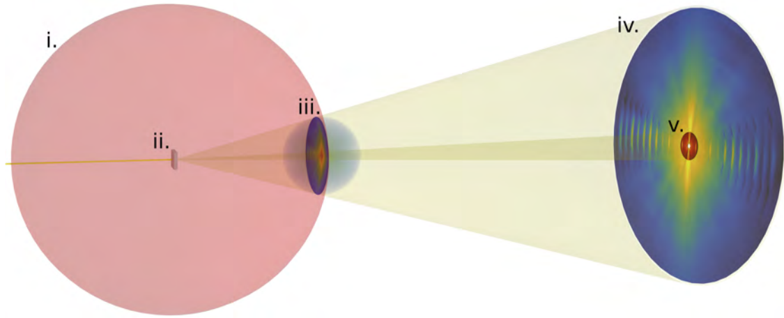
Figure 2.1: Simulation of the effect of the curvature of the Ewald sphere (large red sphere at i.), for when a beam impinges on a sample (small object at ii.). The edge of the Ewald sphere intersects with the origin of the RSM (transparent small sphere at iii.) and the cut of the intersection forms the probed part of the RSM, a curved disk. The outer part of the cut scatters at wide angles, and is greatly magnified when projected onto the detector (large blue-green-yellow iv.). A single circle on the detector forms a small circle of one shell of reciprocal space due to the curvature of the Ewald sphere. The inner part of the cut (dark red area at v.) is much less dramatically magnified as the scattered rays are nearly parallel due to the small scattering angle. A single circle in this part of the detector approximately forms a great circle of a small shell in reciprocal space, due to the small curvature of the Ewald sphere over the angle.
