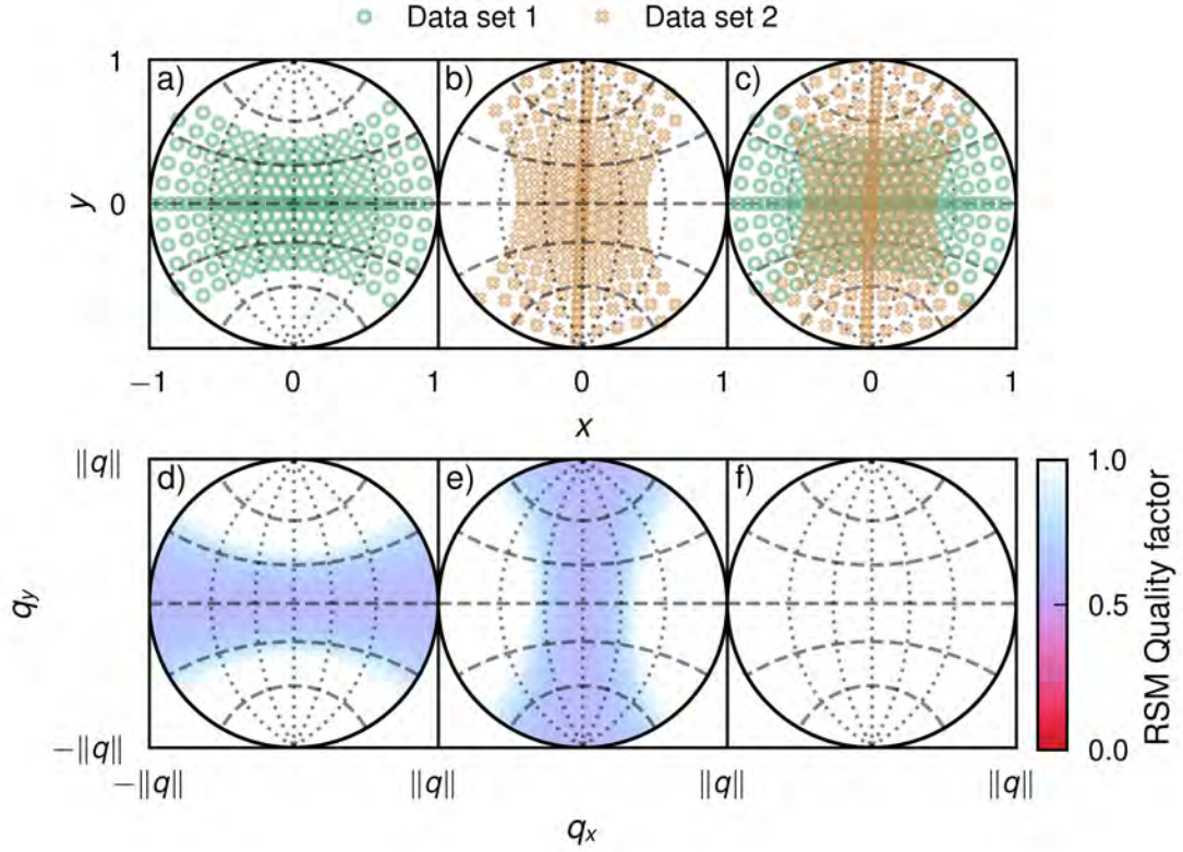
Figure 5.6: Points on hemisphere of projection and theoretical quality factors. a) Probed points on sphere of projection in first measurement. b) Probed points in second measurement. c) Combined points from both measurements. d) Quality factor in reciprocal space from first data set. e) Quality factor from second data set. f) Quality factor from combined data sets.
