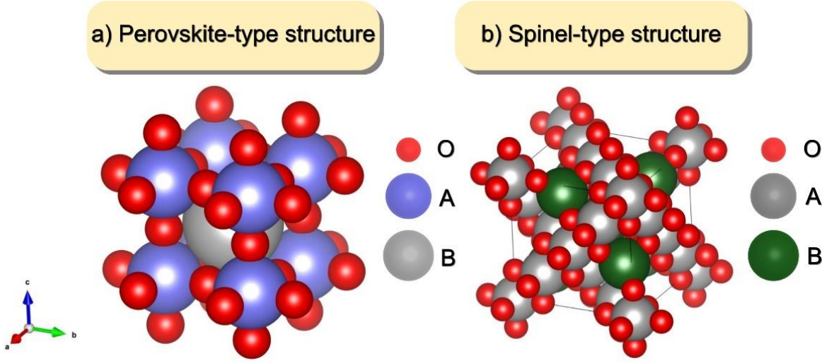
Figure 3.3: Space-filling representation of: a) a Perovskite-type structure; and b) a Spinel-type structure.
