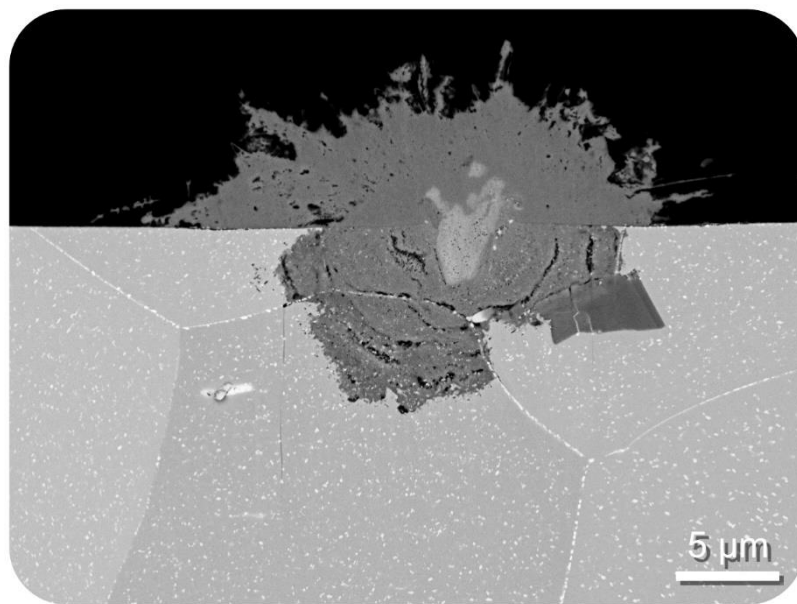
Figure 3.5: Cross-section of a hematite nodule formed on the air-side of a Crofer 22 H foil after exposure in dual-atmosphere conditions (i.e. Ar – 4.8 % \text{H}_2 – 3 % \text{H}_2\text{O} // air – 3 % \text{H}_2\text{O} ) at 600 °C for 336 h.
