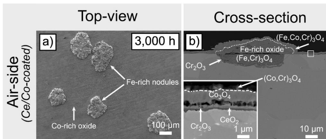
Figure 5.16: Top-view and cross-sectional SEM micrographs of the investigated AISI 441 PVD Ce/Co-coated sample on the air-side, exposed under dual-atmosphere conditions (i.e., Atmosphere 1) at 600 ^{\circ}\text{C} for 3,000 h. Inset: Higher-magnification image of selected scale regions.
