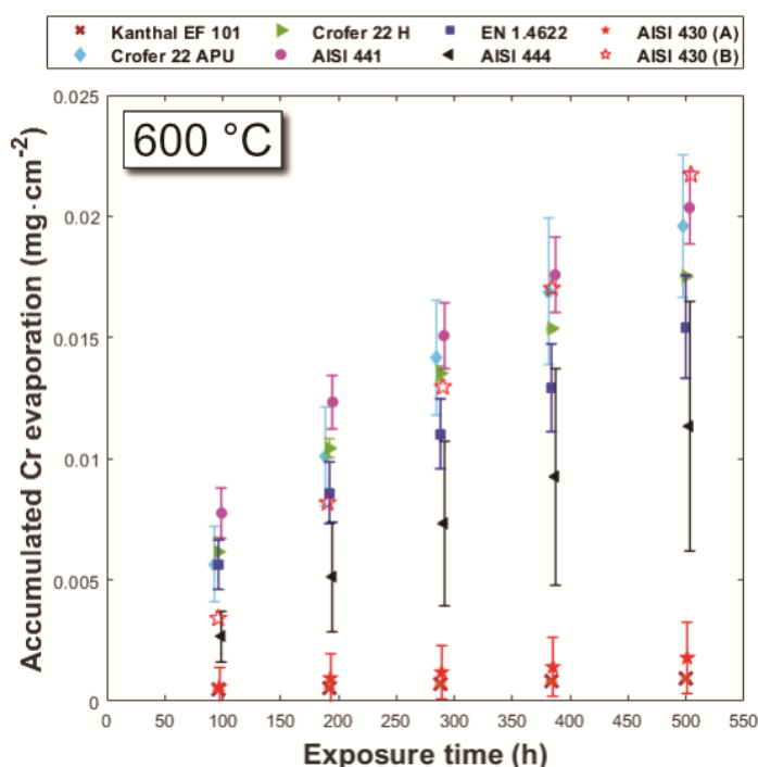
Figure 5.1: Cumulative Cr(VI) evaporation as a function of time for the \text{Cr}_2\text{O}_3 - and \text{Al}_2\text{O}_3 -forming steels exposed at 600^\circ\text{C} for 500 h in air that contained 3 % water vapour. The error bars represent the standard deviation. For Crofer 22 APU and Crofer 22 H, samples from Batch A were used, respectively. The symbols are slightly shifted ( \pm 1 h) to enhance readability.
