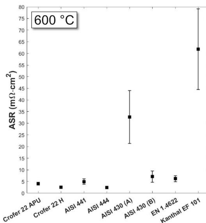
Figure 5.8: ASR measurements performed in air, on different grades of uncoated ferritic stainless steels exposed at 600 °C for 500 h in air + 3 % \text{H}_2\text{O} . Error bars indicate the standard deviation.
