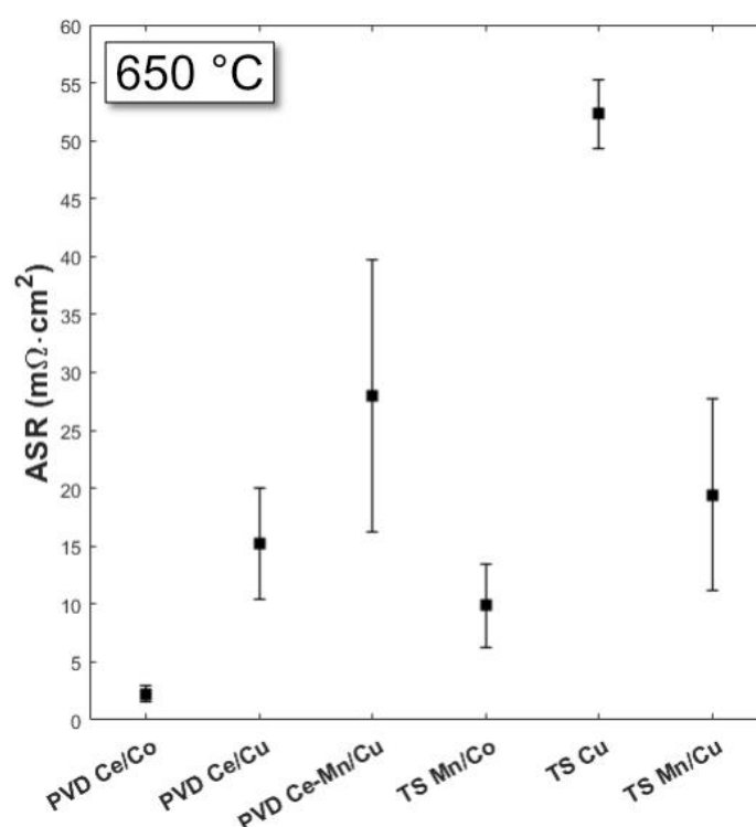
Figure 5.9: ASR measurements performed in air on PVD-coated and TS-coated samples exposed at 650 °C for 1,000 h in air + 3 % \text{H}_2\text{O} . Error bars indicate standard deviation.
