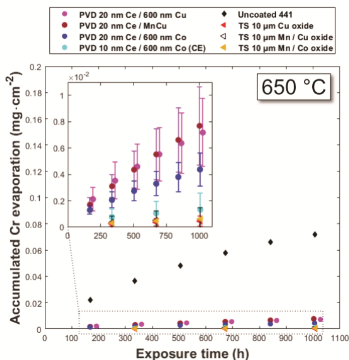
Figure 5.2: Cumulative Cr(VI) evaporation as a function of time for uncoated and coated AISI 441 samples exposed for 1,000 h at 650^\circ\text{C} in air that contained 3 % water vapor. Error bars indicate the standard deviation.
