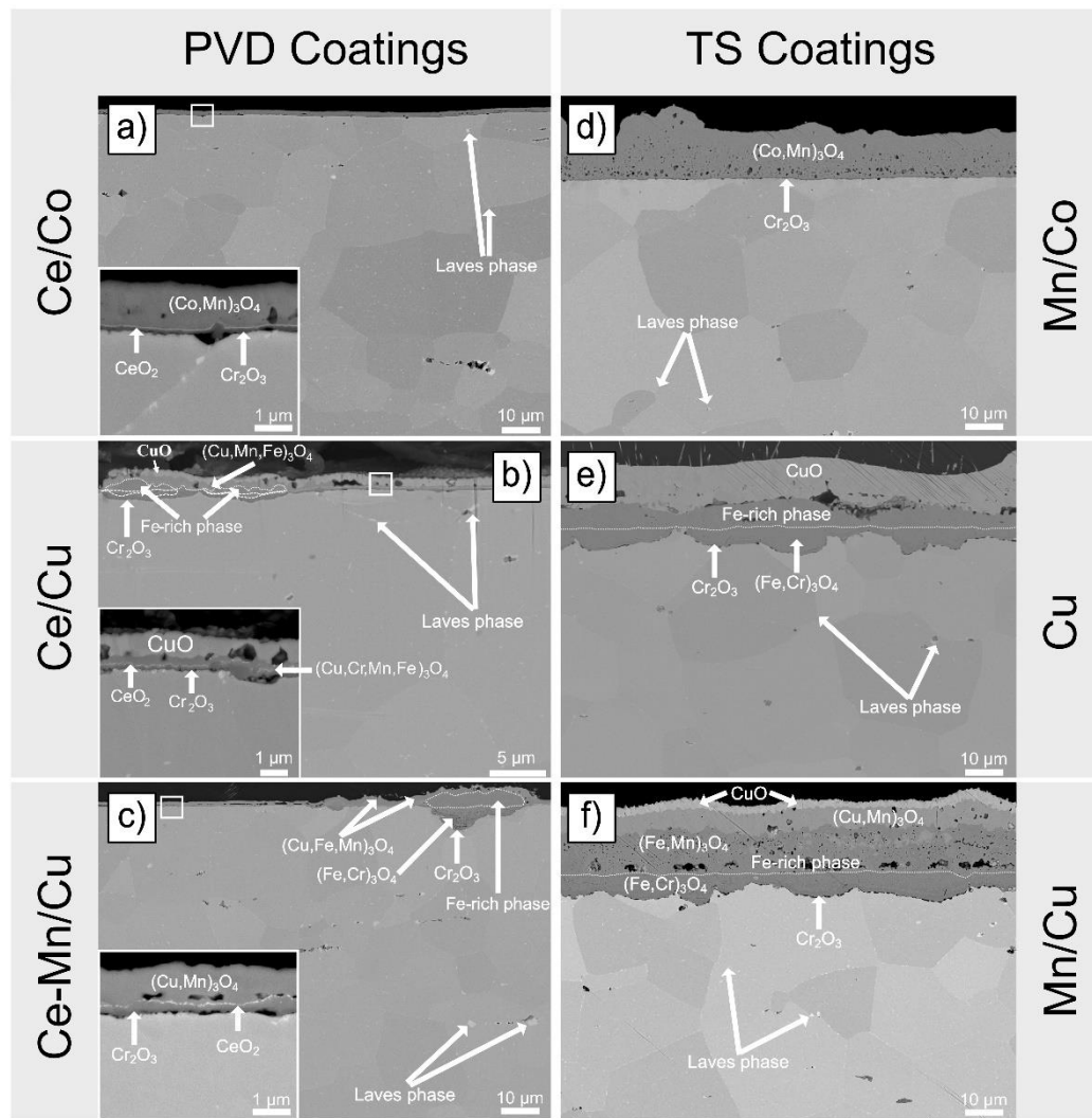
Figure 5.6: SEM Back-scattered Electron (BSE) image of BIB milled cross-section of the investigated PVD and TS coatings exposed to air + 3 % H_2O at 650 °C for 1,000 h.
