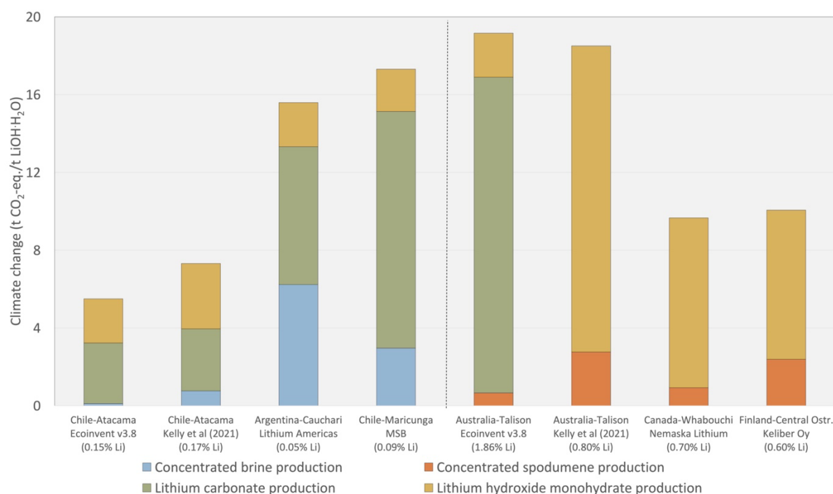
Figure 7. Climate change impacts for different LHM production routes, accounting for geographical locations of the lithium source, the underlying dataset, and the lithium grades.
