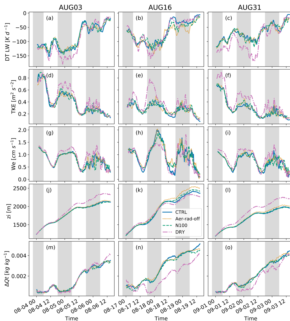
Figure 6. Temporal evolution of the simulated (MIMICA) domain-averaged ( a–c ) LW cooling rate (DT LW) at the MBL top (corresponds to the maximum horizontal domain-averaged LW cooling rate), ( d–f ) MBL TKE, ( g–i ) cloud-top entrainment rate ( W_e ), ( j–l ) inversion height ( z_i ), and ( m–o ) decoupling parameter ( \delta Q_t ). All output variables have 15 min temporal resolution. DT LW and TKE values are smoothed using a 1 h moving average. The entrainment rate is smoothed with a 2 h moving average.
