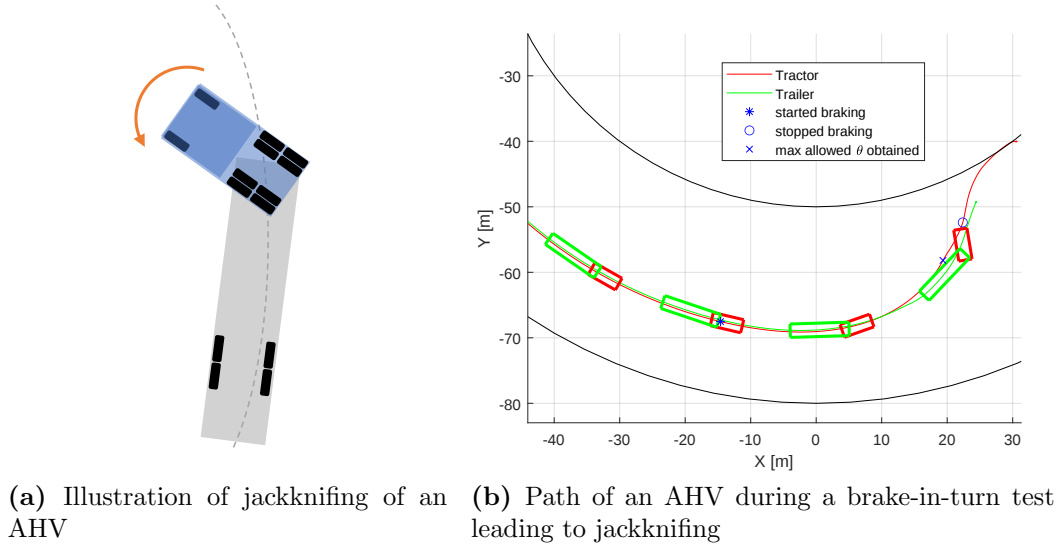
Figure 4.1: Illustration of jackknifing and the corresponding path
