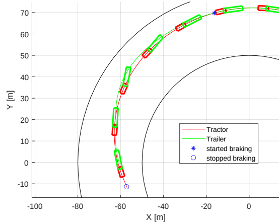
(a) Illustration of trailer swing of an AHV (b) Path of an AHV during a brake-in-turn test leading to trailer swing
