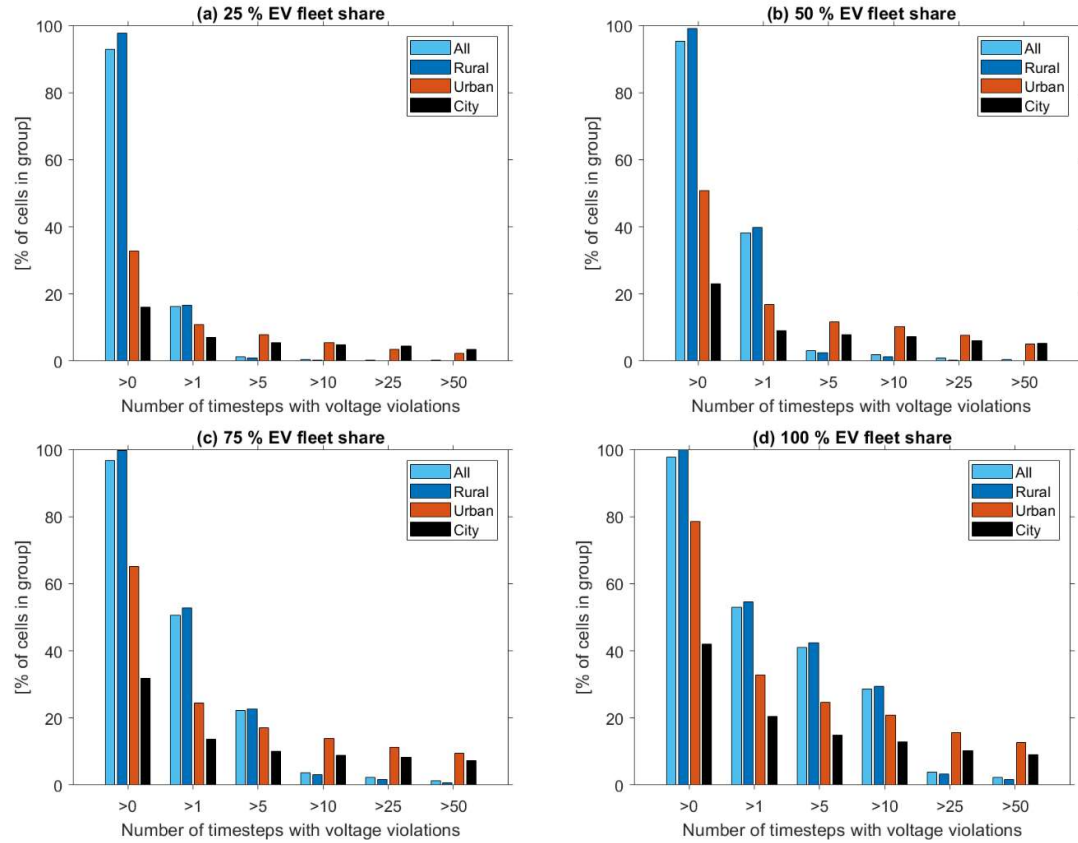
Figure 12. Shares of grid cells with voltage violations in the transformer above a certain value when adding EV charging at four different EV fleet shares: (a) 25%, (b) 50%, (c) 75%, and (c) 100% of the current vehicle fleet electrified for the Direct charging strategy. Panels (a), (b) and (c) represent new results that are not included in the appended papers. The results are shown for rural, urban, and city areas, as well as for all grid cells. The results shown are the average values across all iterations. The results for the 25%, 50%, and 75% EV fleet shares are new results derived for this introductory essay, while the results for 100% EV fleet share are presented in Paper III .
