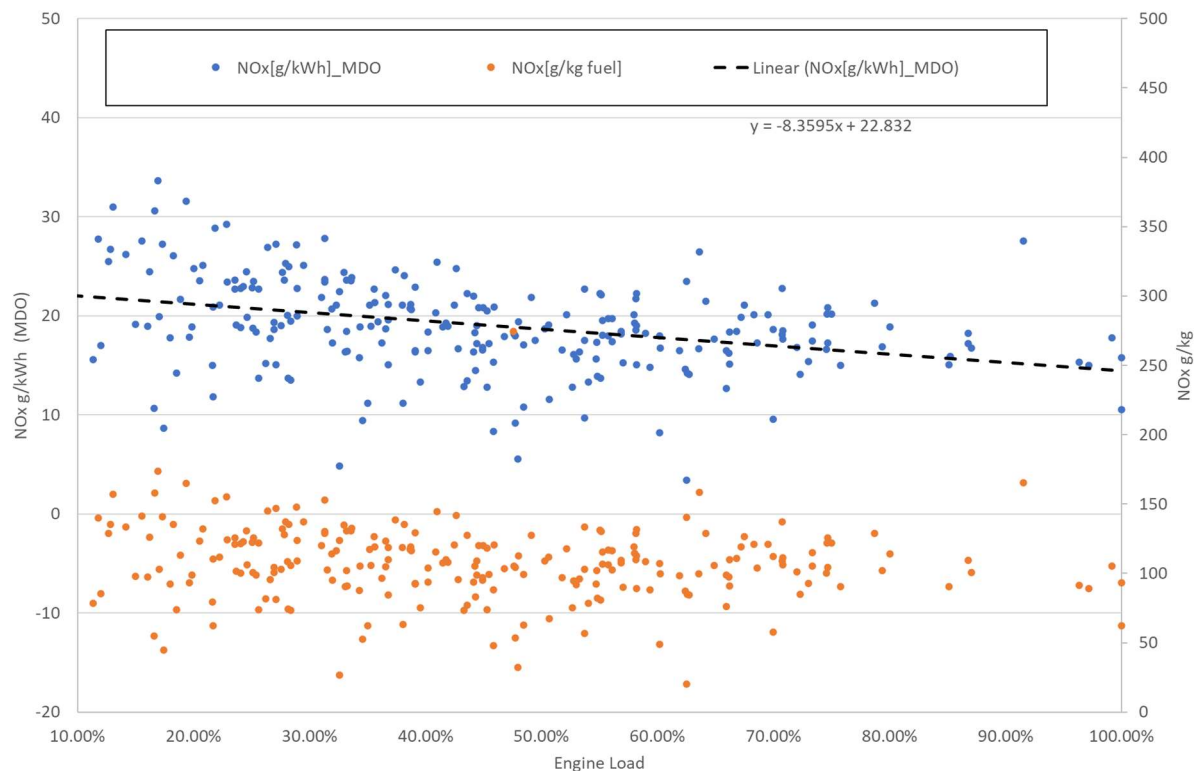
Figure 6 \text{NO}_x measurements of Tier II container ships by an automatic sniffer at the Great Belt bridge Denmark between 2018-2023. A linear fit is also shown to the brake specific \text{NO}_x emission. The Ship engine power was above 20,000 kW and ship lengths were longer than 200 m. The data set includes 248 ships. Note that the Tier II limit for ships with slow speed two-stroke engines is 14.4. g/kWh.
