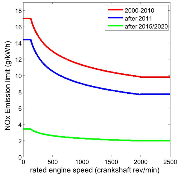
Figure 2 The IMO annex VI \text{NO}_x emission limits for ship engines. The emission levels depend on ship build year, divided into three tiers, and engine type. The engine type is defined according to the corresponding rated engine speed. The emission corresponds to g \text{NO}_x per axial power in kWh, corresponding to a weighted average of several engine loads. Tier III applies in ECAs in North America (ships built in or after 2016) and northern Europe (ships built in or after 2021).
