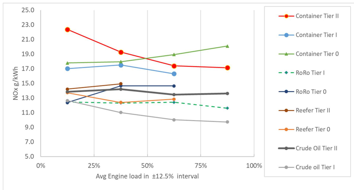
Figure 12 NO x measurements of different ships against engine load by an automatic sniffer at the Great Belt bridge Denmark between 2018-2023.
