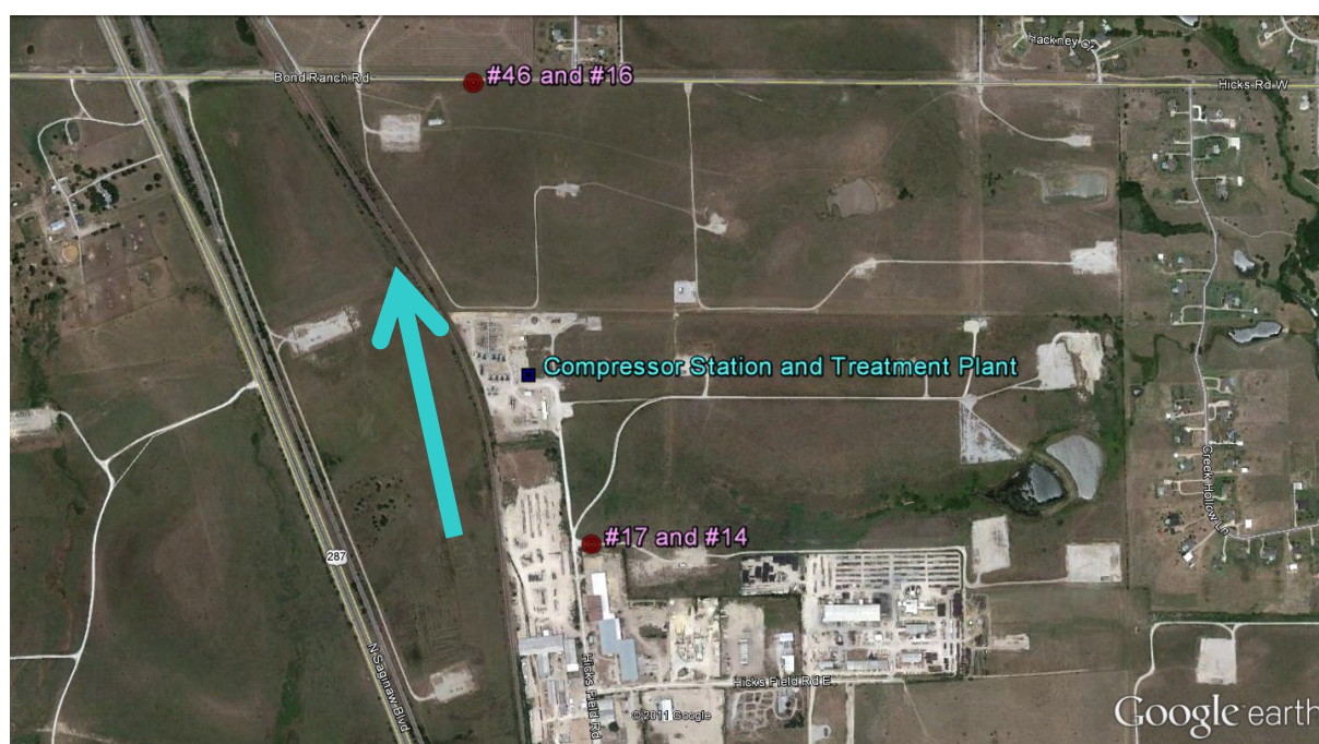
Figure 86 Location of canister samplings downwind (can #46 and #16) and upwind (can #17 and #14) of the Hicks Field Rd compressor station and treatment plant close to Hicks Field Rd. Arrow indicates wind direction.
