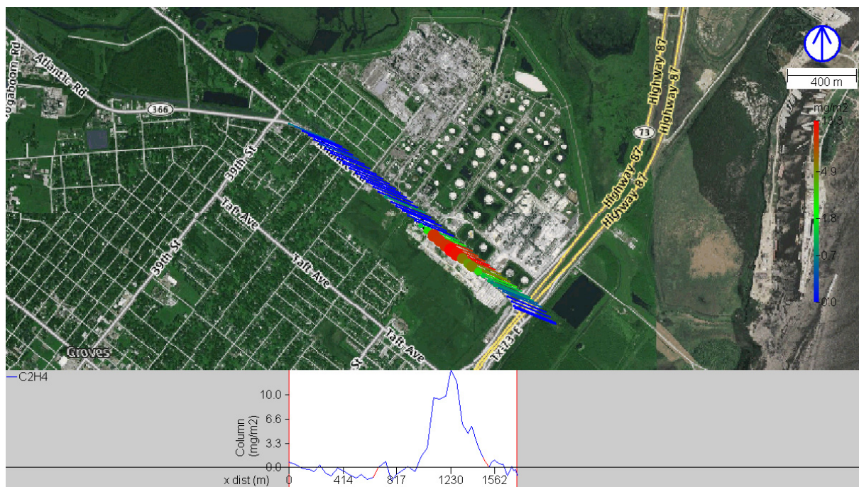
Figure 49 SOF measurement of ethene from area 5 in Port Arthur on May 4, 2011, 16:12–16:18. Each measured spectrum is represented with a point, which color and size indicate the evaluated integrated vertical ethene column. The ethene column by distance driven through the plume is also shown in the lower part of the figure. A line from each point indicates the direction from which the wind is blowing.
