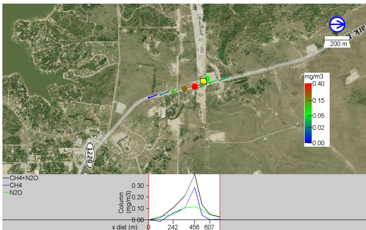
Figure 86 Methane and N2O (tracer) measured by MeFTIR downwind of well pads and a gas distribution system close to Eagle Mt Rd, in the vicinity of the Eagle Mt compressor plant. The emission source is shown in yellow while the tracer release position is shown as a green dot.
