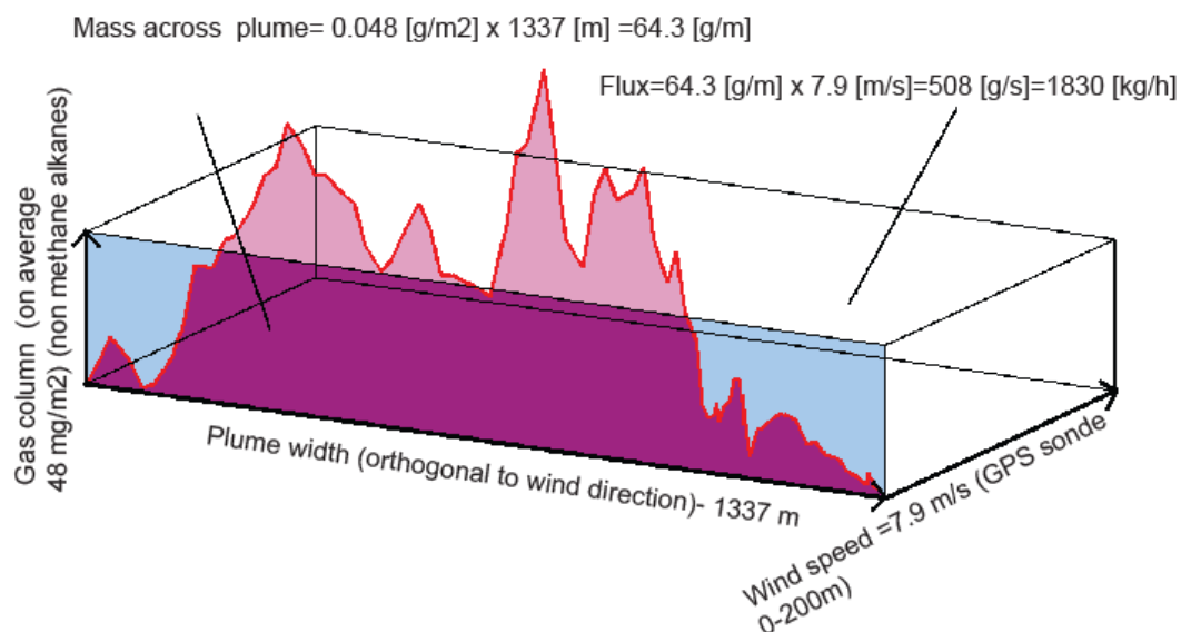
Figure 10 Illustration of the flux calculation in the SOF method for a measurement of alkanes conducted downwind of a refinery. The gas column of alkanes, retrieved from the spectra, is plotted versus distance. In the flux calculation the gas columns are integrated along the measurement transect, corresponding to the lilac area. This area, which is the integrated mass of the plume, corresponds to the same mass as an average column of 48 \text{ mg/m}^2 integrated along the transect of 1337 m. The integrated mass is then multiplied with the wind speed yielding the flux in mass per seconds. Here an average wind speed from ground to 200 m was used corresponding to 7.9 \text{ m/s} obtained from the GPS sonde in Figure 11.
