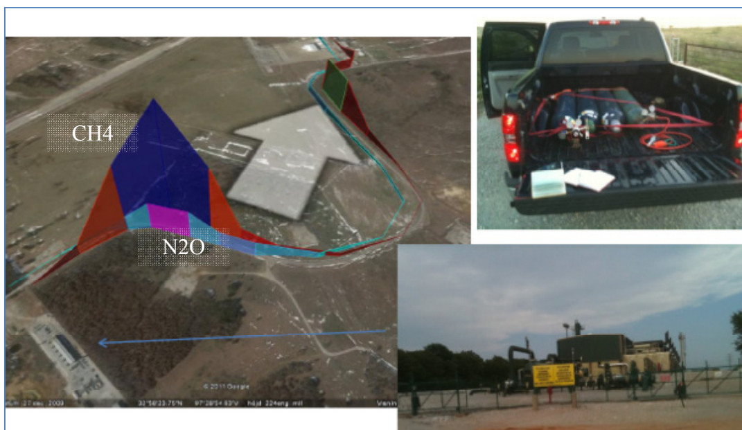
Figure 18 Example of a tracer correlation measurements at a compressor and well pad facility at , 1.8 km SSE of the CAM75 site close to the Kenneth Copeland airfield. The methane (red to blue) and tracer gas (pink to cyan) is shown downwind.
