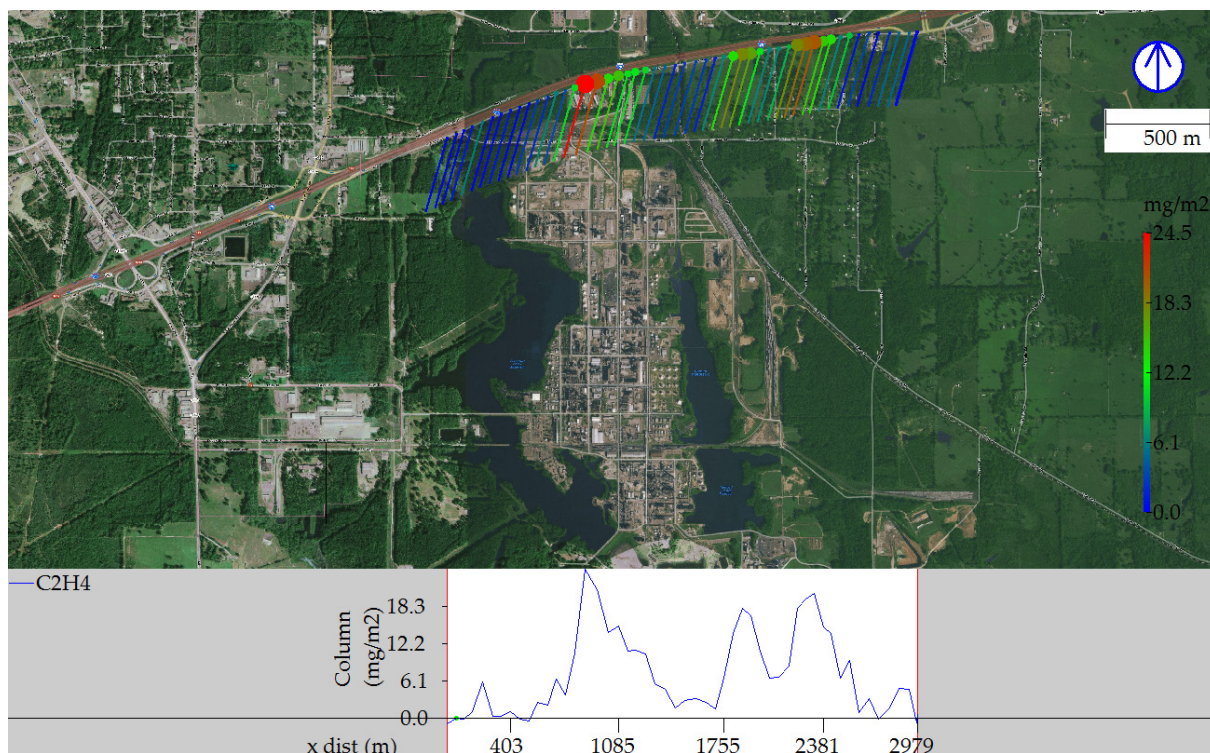
Figure 60 SOF measurement of the ethene emission from the Longview plant on the 7 May 2011, 15:12. Each measured spectrum is represented with a point, which color and size indicate the evaluated integrated vertical ethene column. The ethene column by distance driven through the plume is also shown in the lower part of the figure. A line from each point indicates the direction from which the wind is blowing.
