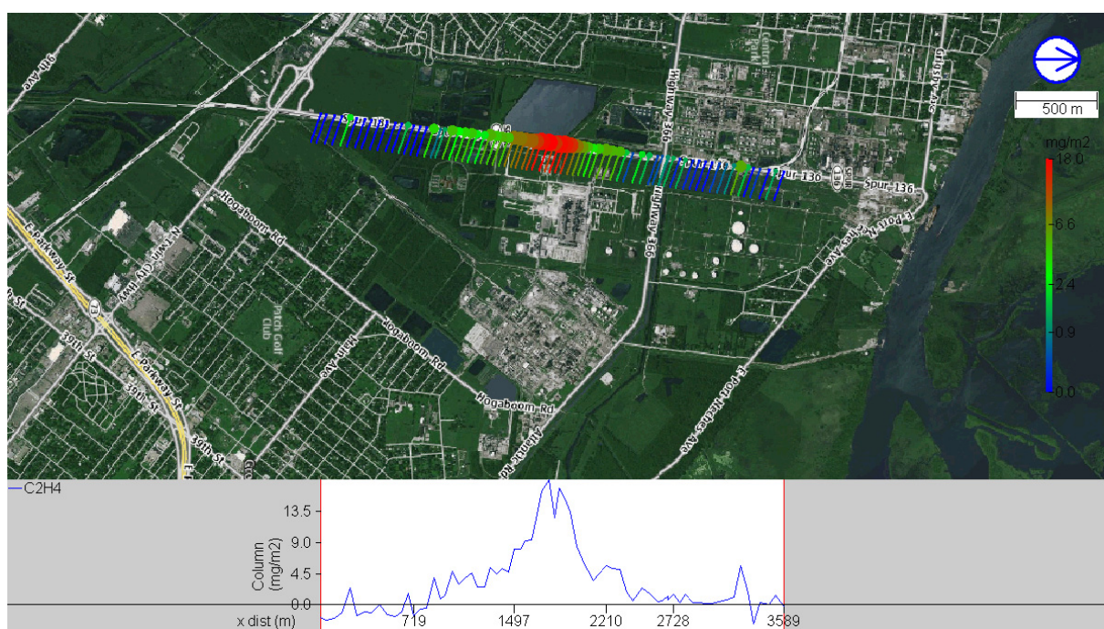
Figure 50 SOF measurement of ethene from area 4 in Port Arthur on May 4, 2011, 17:17–17:25. Each measured spectrum is represented with a point, which color and size indicate the evaluated integrated vertical ethene column. The ethene column by distance driven through the plume is also shown in the lower part of the figure. A line from each point indicates the direction from which the wind is blowing.
