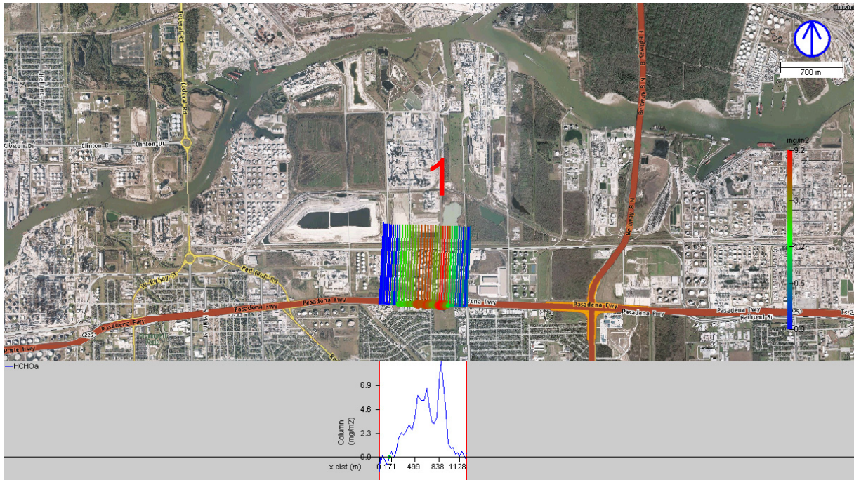
Figure 43 Mobile DOAS measurement of formaldehyde south of the source close to Jefferson Road on April 16, 2011, 12:40–12:42. Each measured spectrum is represented with a point, which color and size indicate the evaluated integrated vertical formaldehyde column. The formaldehyde column by distance driven through the plume is also shown in the lower part of the figure. A line from each point indicates the direction from which the wind is blowing.
