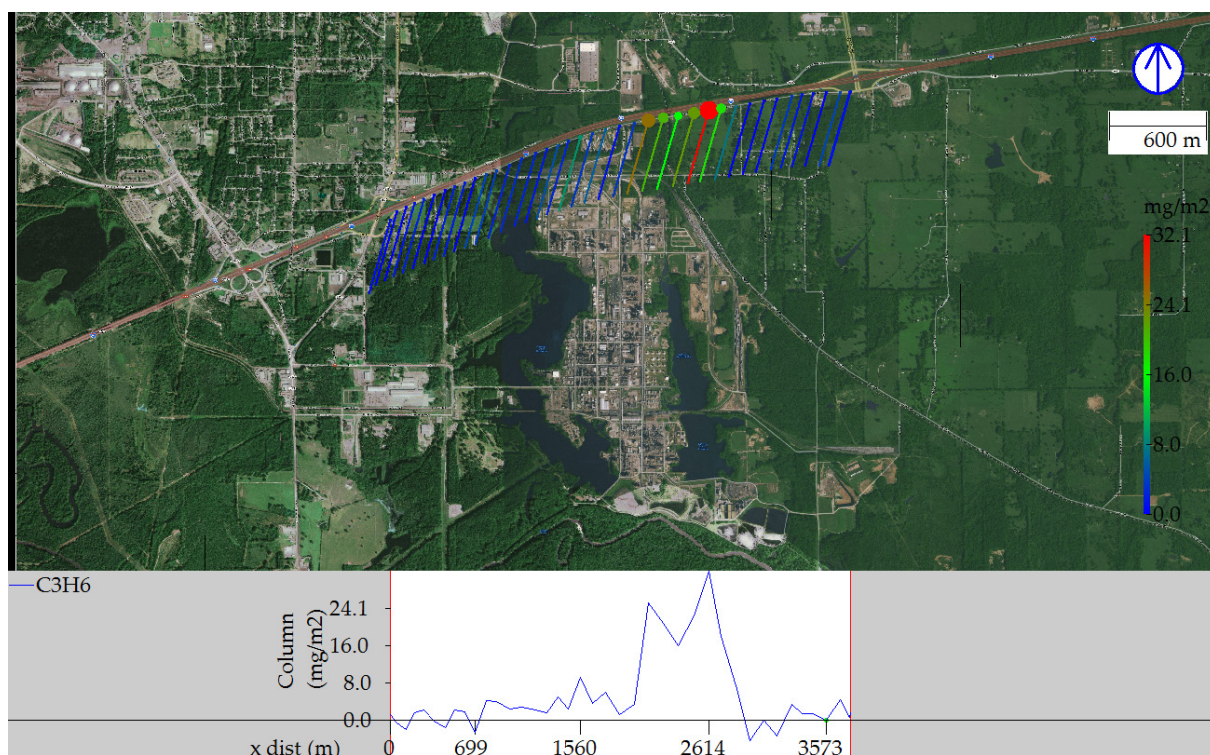
Figure 61 SOF measurement of the propene emission from the Longview plant on the 7 May 2011, 15:36. Each measured spectrum is represented with a point, which color and size indicate the evaluated integrated vertical propene column. The propene column by distance driven through the plume is also shown in the lower part of the figure. A line from each point indicates the direction from which the wind is blowing.
