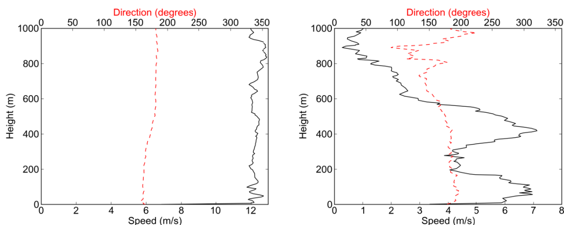
Figure 23 Wind profiles measured with radiosondes. The left profile is from a sonde launched from Baytown at 15:46 on April 23. The right profile is from a sonde launched from Orange, located west of Beaumont/Port Arthur at 17:24 on May 17.
