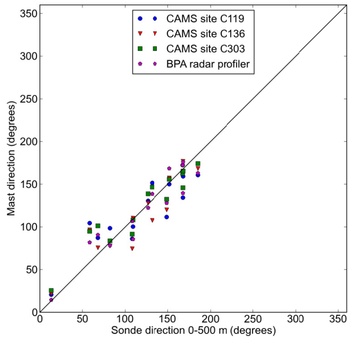
Figure 27 Comparison between wind direction from scaled 10 m high masts and a radar wind profiler; and 0–500 m averages of radiosonde profiles in Beaumont/Port Arthur.
