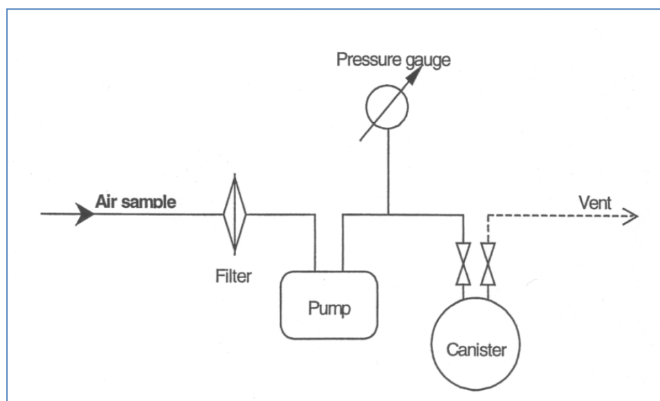
Figure 22 Sampling procedure for 2-valve canisters
