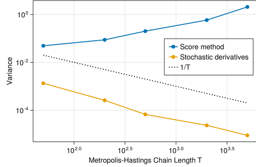
Figure 5. Variance comparison of stochastic derivative-based differentiable MH (Algorithm 2) and score method-based differentiable MH (Algorithm 3), for the Gaussian mixture inference task given in Section 3.1 with the observation H = 0.4 .
