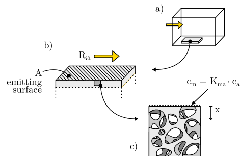
Figure 1. Graphical representation of the model: (a) material placed inside a ventilated room, (b) emitting surface area, (c) internal surface area and interface between material and air.
