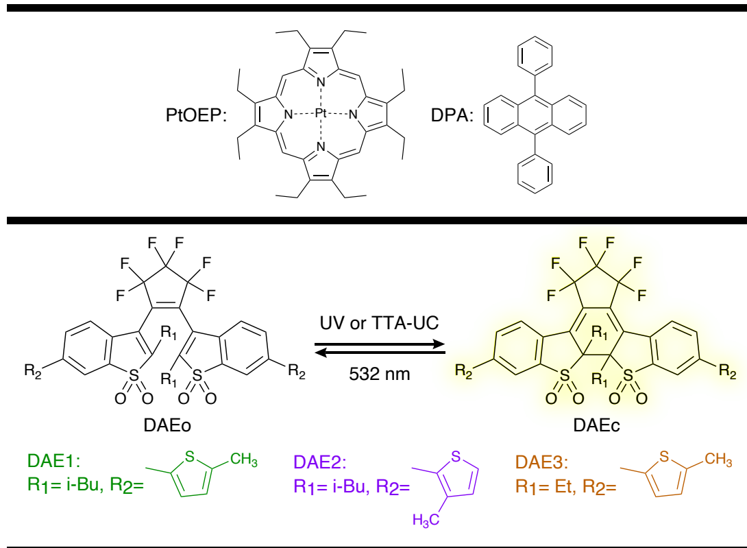
Figure 6.1: Top panel: Structures of PtOEP and DPA. Bottom panel: Structures and isomerization scheme of the three DAEs: DAE1 (green), DAE2 (purple), and DAE3 (brown). UV light or upconverted (TTA-UC) light can be used to isomerize from DAEo to DAEc, and 532 nm light is used to facilitate the reverse isomerization. The yellow glow on DAEc is there to visualize its green light induced fluorescence.
