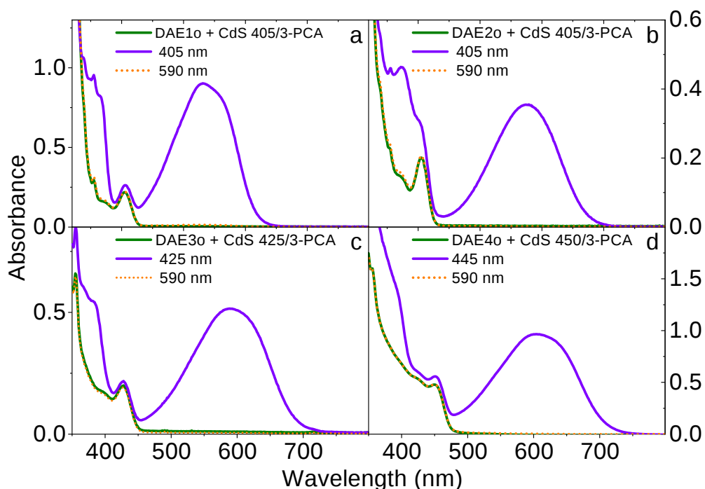
Figure 5.3: Absorption spectra of solutions containing the DAE derivatives (50 \mu\text{M} of a) DAE1, b) DAE2, c) DAE3, and d) DAE4), CdS NCs (0.5 \mu\text{M} CdS 405 in a and b, 0.3 \mu\text{M} CdS 425 in c, and 0.5 \mu\text{M} CdS 450 in d) and 3-PCA (100 \mu\text{M} ) in deaerated toluene. Spectra are recorded for the open isomers before (green lines) and after irradiation of 405 nm, 425 nm, and 445 nm light, respectively (120 s, purple lines), and then after subsequent 590 nm light irradiation (90 s, orange dotted lines).
