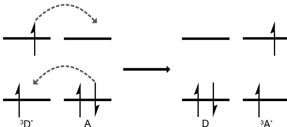
Figure 2.4: Dexter energy transfer depicted as a virtual electron exchange between a triplet excited donor molecule ( ^3D^* ) and a ground state acceptor (A), yielding a ground state donor molecule (D) and a triplet excited acceptor molecule ( ^3A^* ).
