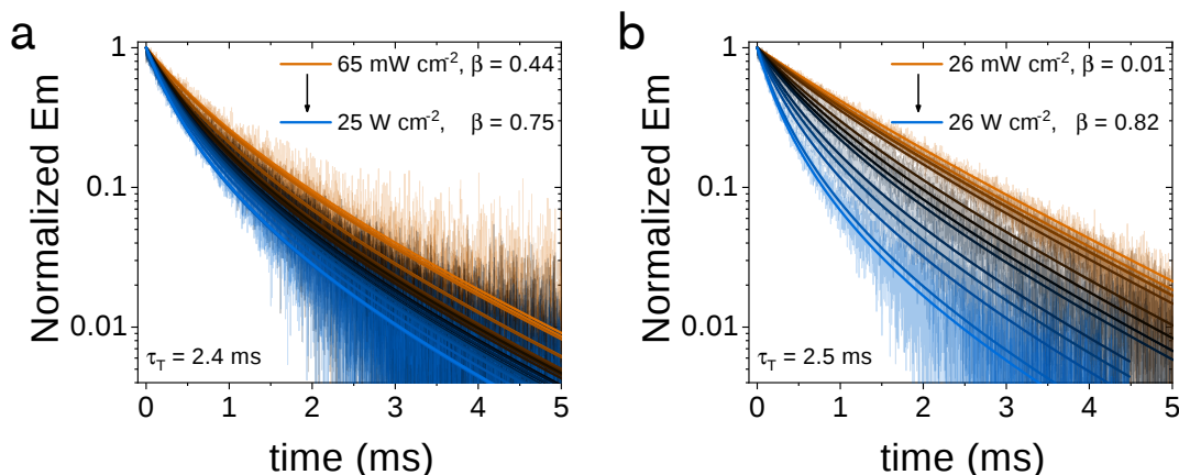
Figure 6.10: Time-resolved upconverted emission of 50 \mu\text{M} PtOEP and 2.0 mM TIPS-An in (a) microcapsules and (b) a glyceryl tri-octanoate solution. Emission was measured at 451 nm (a) and 475 nm (b) upon 532 nm pulsed excitation at various intensities (as indicated in the figures). The fitting lines represent the best global fits of Equation (3.5), employing a shared \tau_T .
