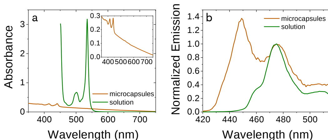
Figure 6.9: Steady-state absorption (a) and emission ( \lambda_{ex} = 532 nm, 20.0 mW) (b) spectra of 50 \mu M PtOEP and 2 mM TIPS-An upconversion solutions in PLGA/glyceryl trioctanoate microcapsules (brown) and in a glyceryl trioctanoate solution (green). The inset in (a) provides a magnified view of the absorbance spectrum for the microcapsule sample. Both samples were measured in 10 mm x 10 mm cuvettes.
