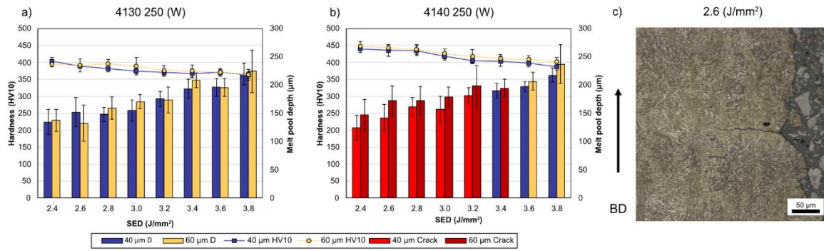
Figure 9. Hardness (HV10) and melt pool depth (μm) as a function of SED (J/mm²) for a) 4130 and b) 4140 at 250 (W) laser power. Specimens containing cold cracks are coloured red.
