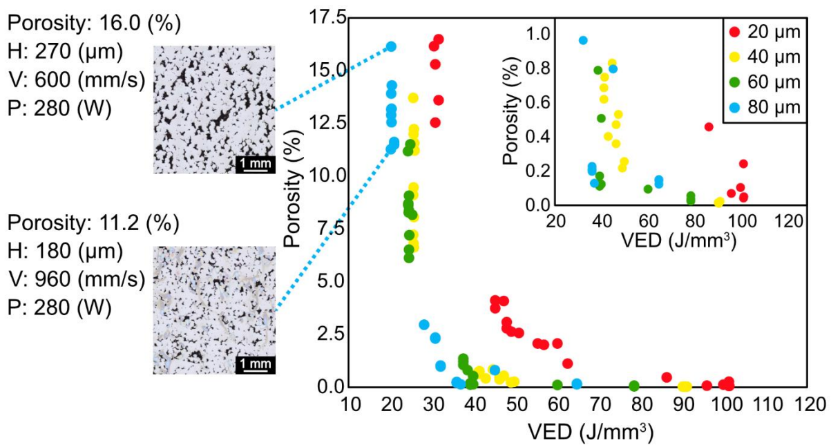
Figure 11. Influence of the combined process parameter VED \text{J/mm}^3 on porosity evolution at 20, 40, 60 and 80 \mu\text{m} layer thickness.
