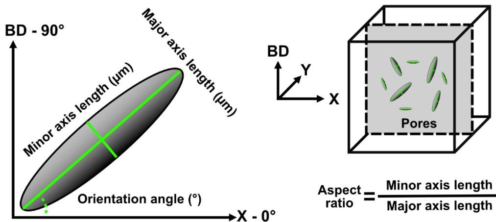
Figure 6. Pore characteristics of interest in paper 2.
