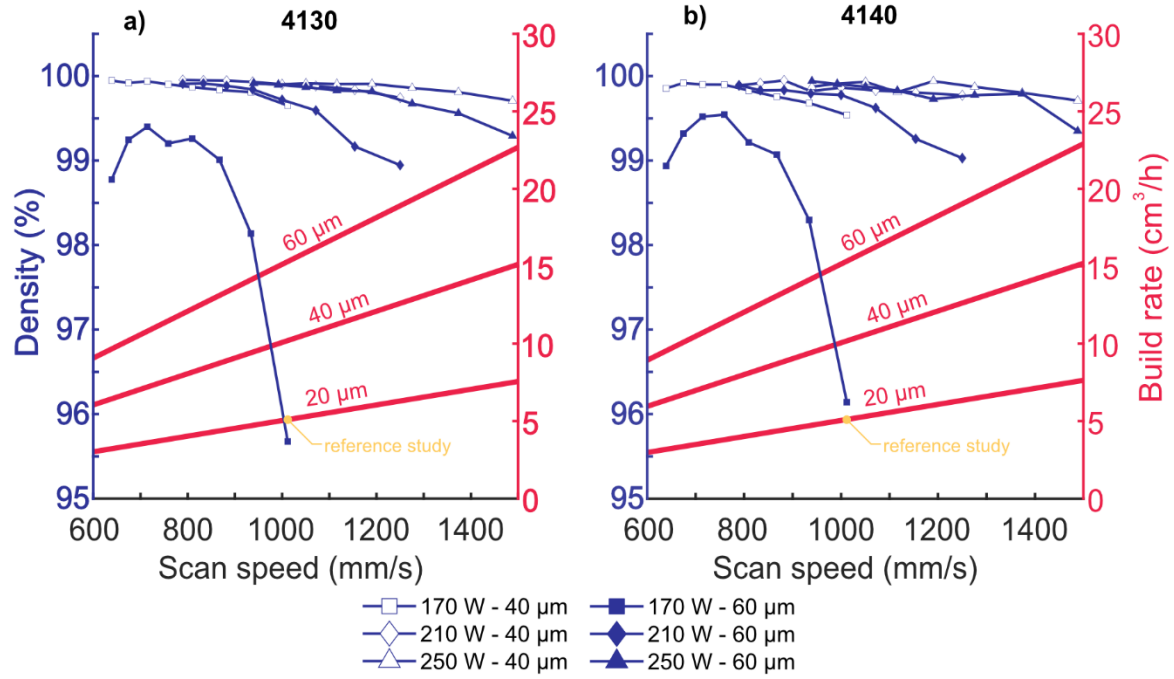
Figure 10. Density (%) as a function of scan speed (mm/s) and build rate (cm³/h) for a) 4130 and b) 4140 produced samples. Solid lines of constant build rate (cm³/h) are presented on the secondary y-axis and corresponds to the density measurements by layer thickness 40 μm and 60 μm. For each density measurement the build rate can be read from the solid lines for the corresponding layer thickness at that scan speed. The achieved build rate with the same machine and alloy in previous study [33] is plotted in yellow as a reference value at 20 μm layer thickness.
