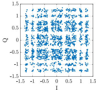
Figure 2.5: Illustration of how an SOP rotation with \theta = \pi/8 affects one of the polarizations in a dual polarization transmission of 2000 16QAM symbols.
