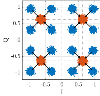
Figure 3.3: Constellation transformation of 16QAM to QPSK with the decision boundaries marked with dotted lines.
