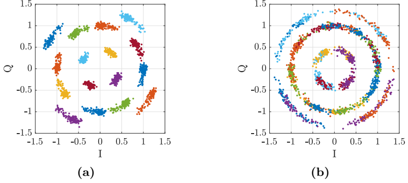
Figure 2.6: Illustration of how phase noise affects a 10 GBaud transmission of 2000 16QAM symbols, for (a) \Delta v T_s = 10^{-5} ( \Delta v = 100 kHz) and (b) \Delta v T_s = 10^{-6} ( \Delta v = 1 MHz).
