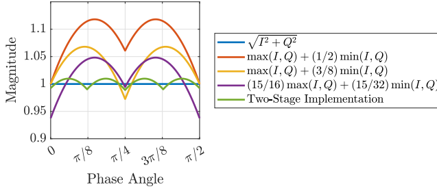
Figure 4.4: Magnitude calculated using different parameter settings for the \alpha \max + \beta \min approximator.
