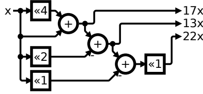
Figure 4.3: Example of MMCM.
