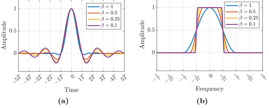
Figure 2.3: Raised cosine (a) impulse and (b) frequency response for different roll-off factors.
