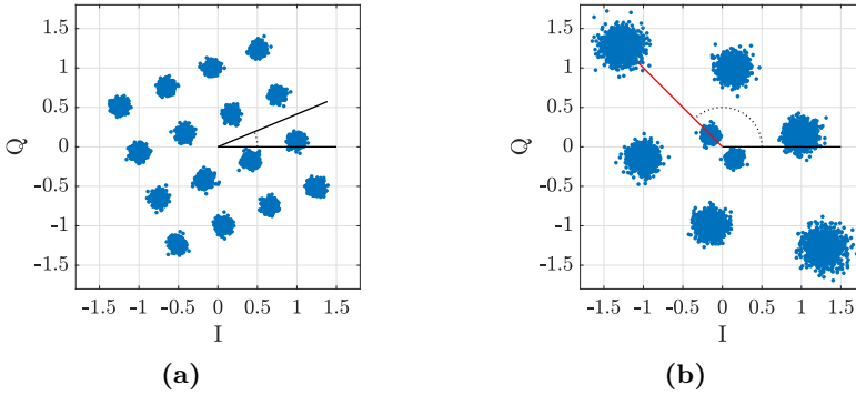
Figure 3.4: Assuming 16QAM input symbols to the principal component phase estimator, shown in (a), (b) shows the squared input symbols, with the principal component marked with a red line
