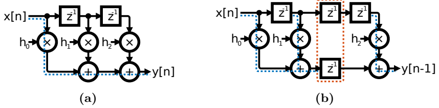
Figure 4.1: A three-tap FIR filter shown (a) without pipelining and with the critical path indicated by a blue dashed line, and (b) with one stage pipelining marked with an orange dashed square. Note that the pipelined version has three approximately equal shorter critical paths.
