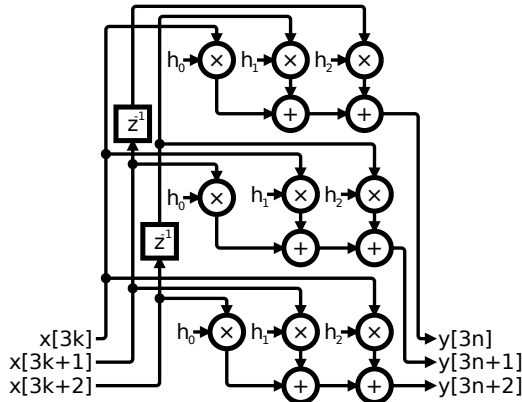
Figure 4.2: Three-tap FIR filter parallelized in three lanes.
