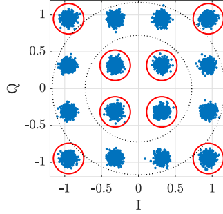
Figure 3.2: 16QAM constellation with the Class-1 symbols circled and the amplitude boundaries marked with dotted lines.
