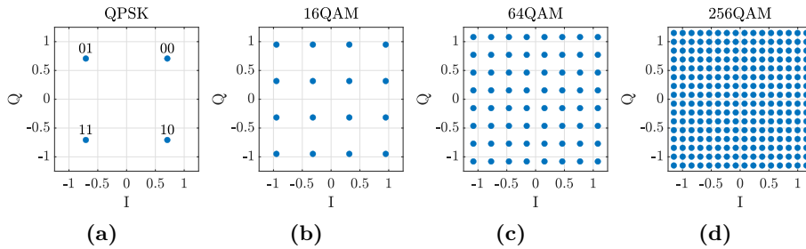
Figure 2.1: Constellation diagram of (a) QPSK, also showing the encoded bit values, (b) 16QAM, (c) 64QAM and (d) 256QAM.
