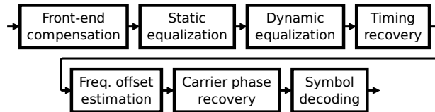
Figure 3.1: Typical architecture of a coherent DSP.
