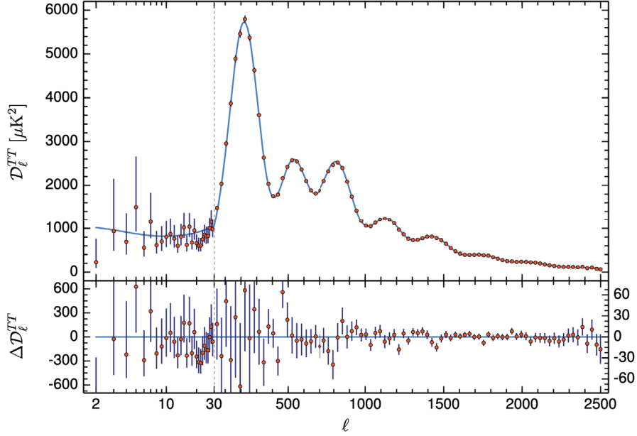
Figure 2.1: The CMB power spectrum taken from Planck 2018 [1]. The blue line is the theoretical prediction from \Lambda CDM with the best fit cosmological parameters given in eq. (2.11), and the red dots are the values inferred from the measurements of the CMB with 1\sigma error bars. The upper panel shows the spectrum, whereas the lower panel shows the discrepancy between the theoretical prediction and the measured result. Note that the horizontal scale changes from logarithmic to linear at the vertical dashed line at \ell = 30 , and that also the vertical plot range in the lower panel is reduced by a factor of 10 to the right of the line.
