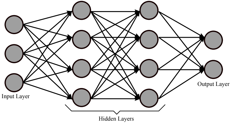
Figure 3.2: Illustration of MLP, i.e. feedforward fully connected neural network.
