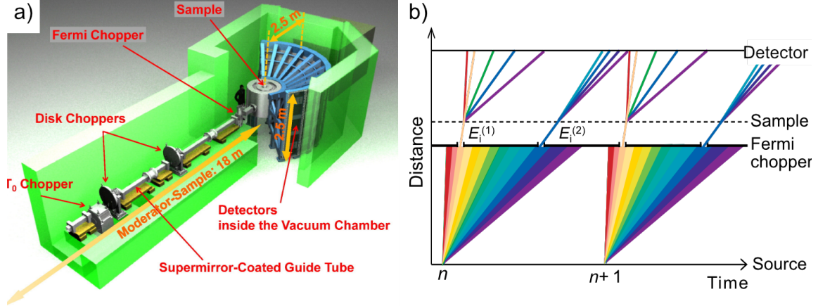
Figure 4.3: (a) Schematic view of the spectrometer 4SEASONS at J-PARC [63]. (b) Time distance diagram illustrating the ToF technique for a direct-geometry spectrometer at a pulsed source (adapted from [58] with permission of The Licensor through PLSclear).
