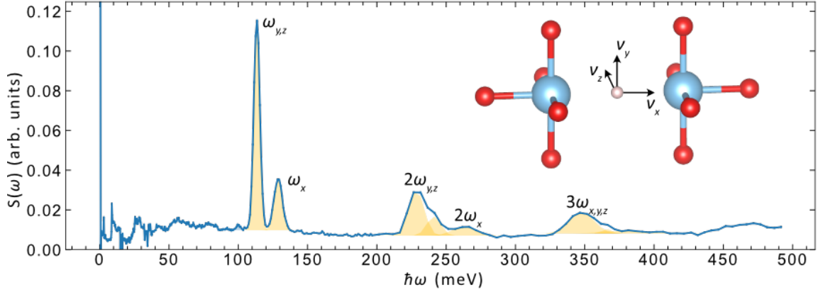
Figure 3.4: INS spectrum of a powder sample of \text{BaTiO}_{2.9}\text{H}_{0.1} measured on LA-GRANGE at the ILL, together with fits of the hydrogen peaks (shaded areas). Inset: illustration of the directions of the three vibrational modes in \text{BaTiO}_{3-x}\text{H}_x .
