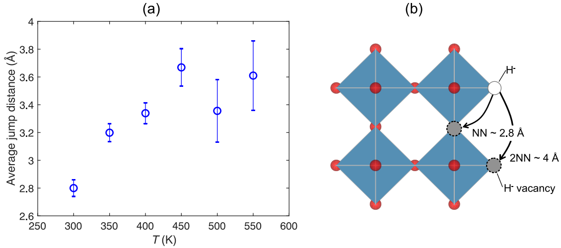
Figure 6.3: (a) Temperature dependence of the hydride-ion jump distance on BaTiO 2.55 H 0.12 . (b) Illustration of the two jump mechanisms involved. The Ba ion is omitted for clarity. Ti, O and H are represented by blue, red, and white spheres.
