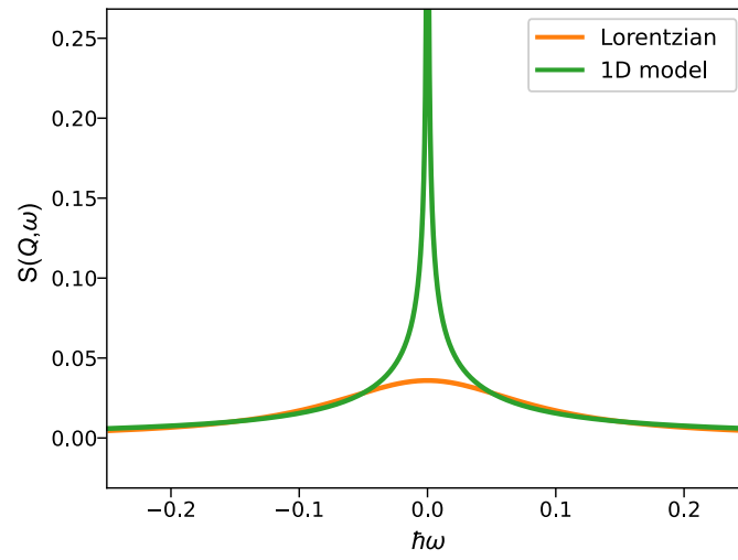
Figure E.1: Comparison of the S(Q, \omega) lineshape between an isotropic diffusion [eq. (3.13)] and 1D diffusion [eq. (E.1)].
