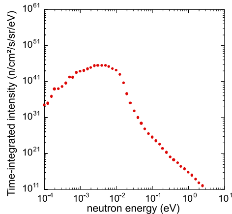
Figure 4.2: Spectral intensity of the neutron pulses after the coupled hydrogen moderator. Adapted from [62].
