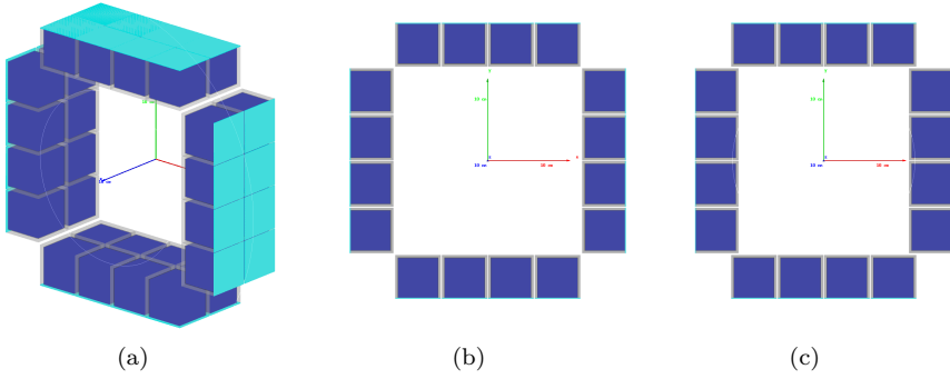
Figure 4.18: Box with 2 rings (16 crystals in each ring, for a total of 32). (a) Without overlap, side view. (b) Without overlap, face view. (c) With overlap, face view.
