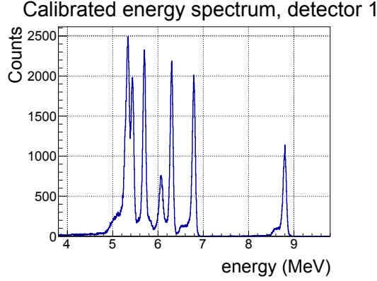
Figure 3.5: Calibrated energy spectrum from detector 1.
