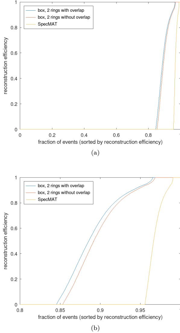
Figure 4.19: Detection efficiency for different configurations. The efficiency is calculated for each event as the registered energy divided by the originally emitted \gamma energy. The events are then sorted by efficiency. The left plot shows all events. On the right, the region with non-zero energy deposits is shown.
