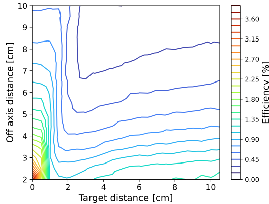
Figure 4.14: Efficiency map for a luminosity detector consisting of four position-sensitive silicon detectors mounted parallel to the beam-line, with the active surface oriented such that they face the beam axis, as a function of the off-axis distance and distance to the target plane. Figure from Ref. [50].
