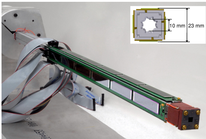
Figure 3.2: The HELIOS silicon-detector array. Six detectors are mounted on each of the four sides. The target would be in the lower-right corner of the picture. For the ^{238}\text{U}(\text{d},\text{p}f) experiment, the distance between the array and the target was 55 mm. The red piece in front shields the array from low energy protons which complete multiple turns in the magnetic field before hitting the array (multi-turn protons). Figure from Ref. [13].
