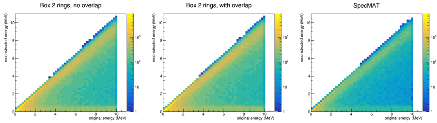
Figure 4.20: Doppler-corrected vs simulated \gamma energy for a box with 2 rings without and with overlap, and SpecMAT. Except for the total efficiency differences between the configurations, the Doppler-corrected energies look very similar.
