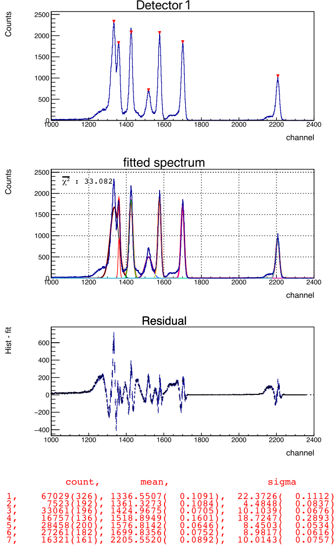
Figure 3.4: The first step of fitting of the c_t spectrum is illustrated in the following manner: the top plot shows peaks identified using the Search method from the ROOT [30] TSpectrum class; the middle plot displays the fitted spectrum (at most maximum 7 separately fitted peaks as well as their sum); the lowest plot exhibits the original c_t spectrum with the subtracted fitted function. Parameters for each individual peak, along with their corresponding errors, are provided below the plots.
