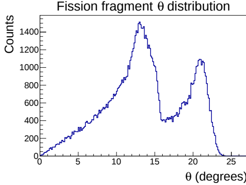
Figure 4.8: Angular distributions of ^{230}\text{Ac} fission fragments simulated by GEF and boosted to the beam frame. For the simulated ^{229}\text{Ac} beam energy of 8 MeV/u, two peaks around 13^\circ and 21^\circ can be distinguished, corresponding to heavy and light fission fragments, respectively.
