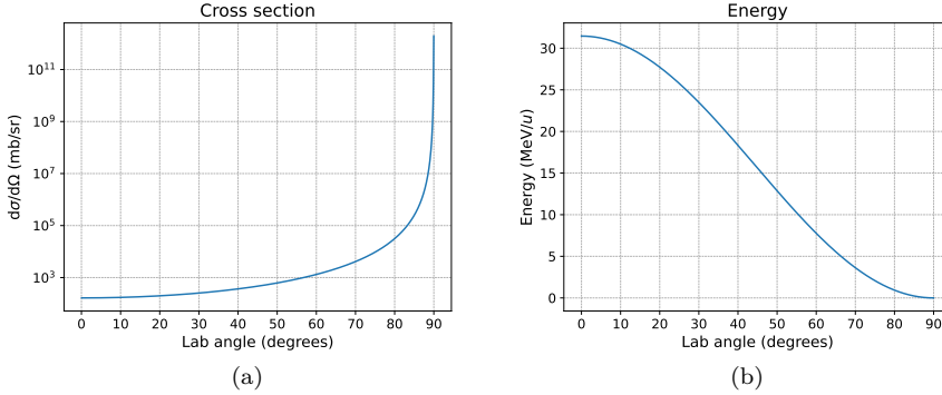
Figure 4.10: (a) Cross section of deuterons ejected from the target when ^{229}\text{Ac} of 8 \text{MeV/u} impinges as a function of the lab angle. (b) Energy of the scattered deuterons as a function of the lab angle.
