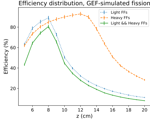
Figure 4.9: Geometric efficiency of the CD-shaped fission fragment detector at a beam energy of 8 MeV/ u as a function of its distance to the target. The detector has inner and outer radii of 11 mm and 35 mm, respectively. The dotted blue line represents the efficiency of detecting only the light fission fragment, the dashed orange line corresponds to the efficiency of detecting only the heavy fragment, and the solid green line illustrates the efficiency for detecting both fission fragments in coincidence. Figure from Ref. [50].
