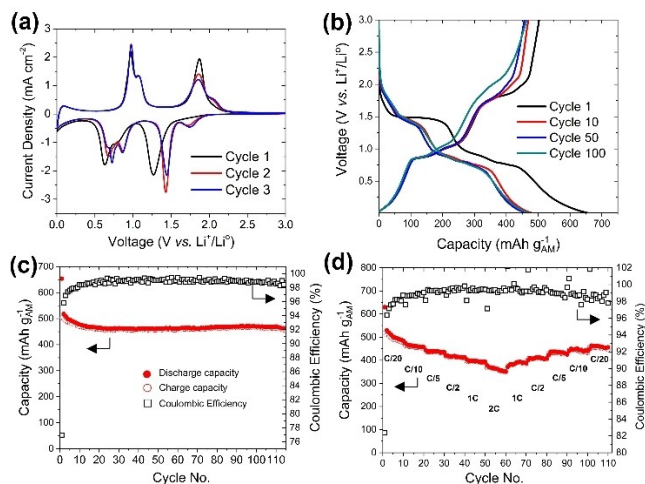
Figure 2. BSST anode half-cell tests: (a) CV ( 0.1 \text{ mVs}^{-1} ), (b) GC discharge-charge profiles (C/20), (c) GC (C/20), and (d) rate capability.
