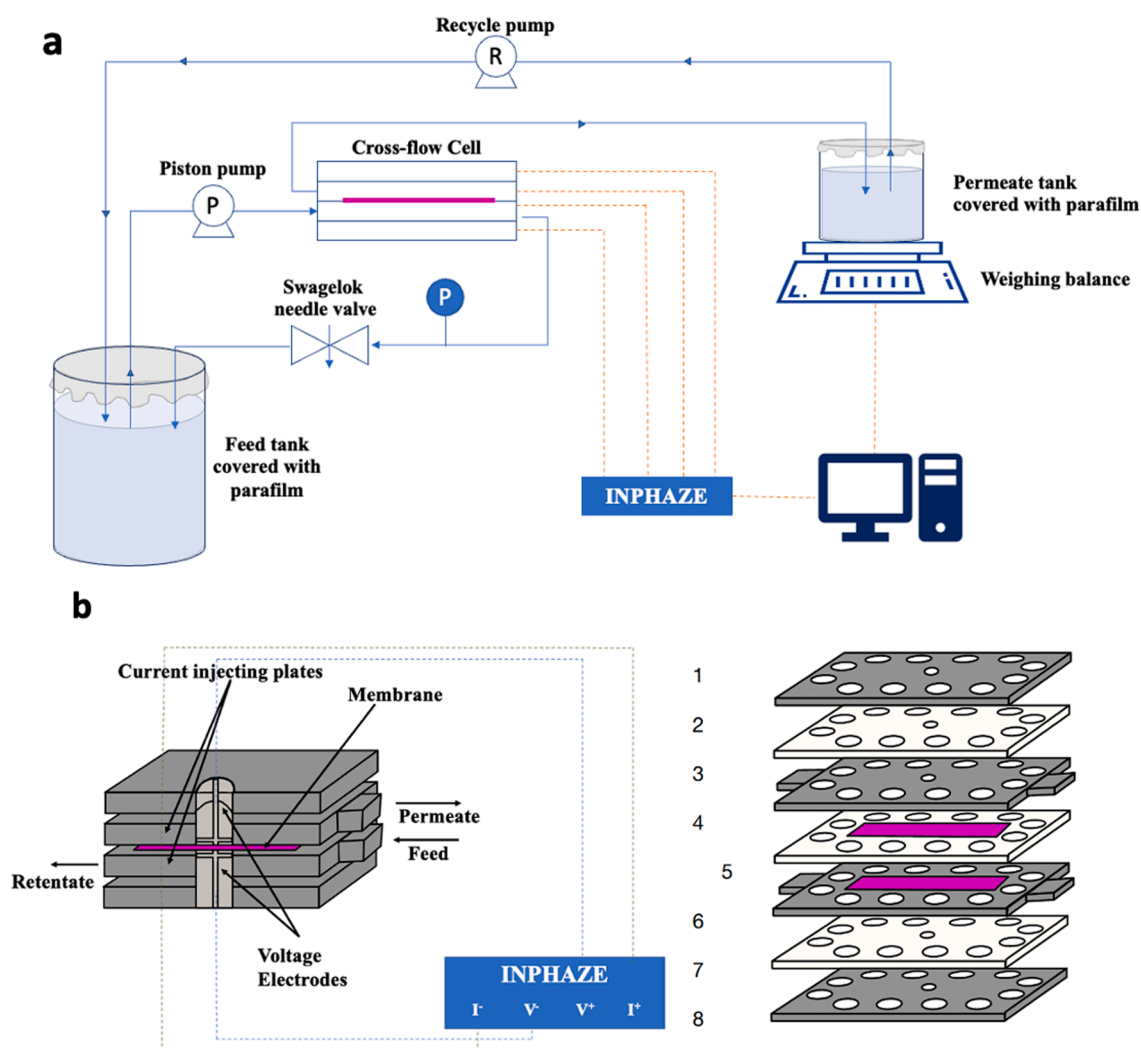
Fig. 1. (a) Crossflow NF filtration setup with real-time EIS monitoring; and (b) cross-section of the crossflow NF-EIS membrane cell linked to the INPHAZE™ spectrometer. 1,3,6 and 8 are stainless steel plates; 2, 4 and 7 are insulating plastic plates and 5 is the membrane. 4 has the hole in the middle which is in the shape of the membrane to provide the structural support to hold the membrane in place during the filtration experiment. 4 helps to establish a fix distance between the membrane and the electrodes such that the active surface area of the membrane is always in contact with the fixed amount of solvent and metals plates 3 and 6.
