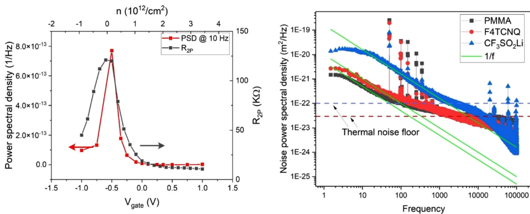
FIG. 3. (a) Comparison of two-point resistance ( R_{2P} ) and noise power spectral density amplitude (at f = 10\ \text{Hz} ) measured for electrostatically gated epigraphene. Negative charge carrier density corresponds to the p type of carrier. (b) Comparison of noise power spectral density (PSD) of PMMA ( n = 7 \times 10^{12}\ \text{cm}^{-2} ), F4TCNQ ( n = 0.42 \times 10^{12}\ \text{cm}^{-2} ), and \text{CF}_3\text{SO}_2\text{Li} ( n = 0.4 \times 10^{12}\ \text{cm}^{-2} ). PSD is normalized with respect to device geometry. For \text{CF}_3\text{SO}_2\text{Li} , the values correspond to the gate voltage fixed at the Dirac point.
