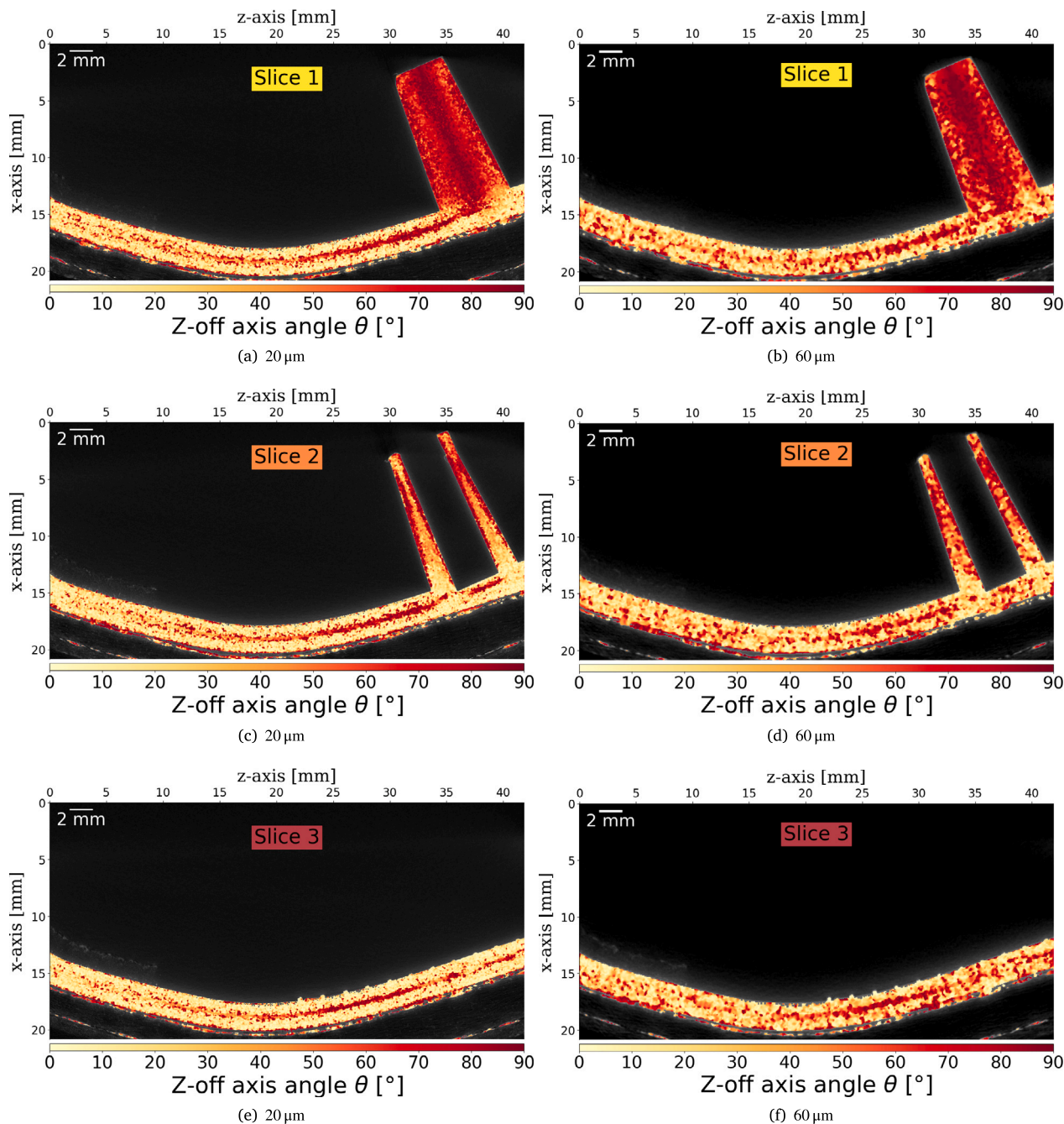
Fig. 7. Comparison of the z-off axis (zenith) angle \theta colour-mapped onto the original grey-scale images for Slice 1–3 in the Dome Scan for the two voxel-sizes 20 μm and 60 μm.
