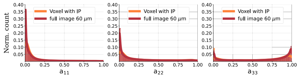
Fig. 13. Histograms of the three a_i components of the second-order orientation tensor (Eq. (8)) computed for the full three-dimensional image data-set (207,660,459 voxels with a voxel-size of 60\ \mu\text{m} ) and for 43,180 voxels which spatially contain an integration point (IP). Note, each second-order orientation tensor (Eq. (8)) is computed based on one dominant fibre orientation vector p . Both counts in the histogram are normalised for better comparison. The solid lines represent Gaussian Kernel density estimations.
