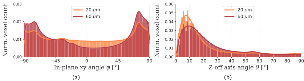
Fig. 8. Histograms of the in-plane xy (azimuthal) angle \phi (a) and z-off axis (zenith) angle \theta (b) for the Rib Scan for the two voxel-sizes 20 μm and 60 μm. The solid lines represent Gaussian Kernel density estimations. The voxel counts are normalised for better comparison.
