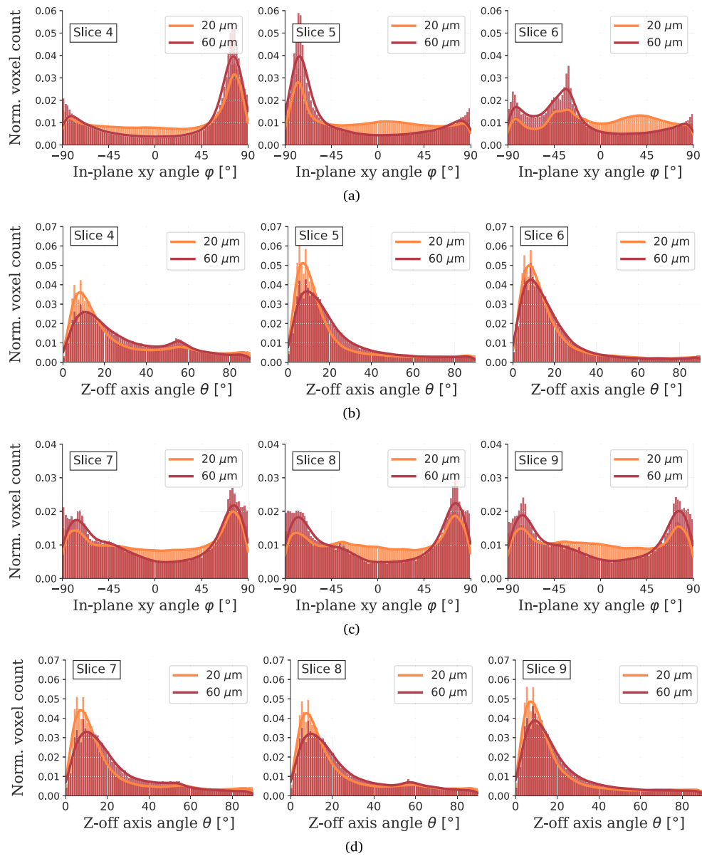
Fig. 9. Comparison of the in-plane xy (azimuthal) angle \varphi (a) and (c) and z-off axis (zenith) angle \theta (b) and (d) for Slices 4–9 in the Rib Scan and the two voxel-sizes 20\ \mu\text{m} and 60\ \mu\text{m} . The solid lines represent Gaussian Kernel density estimations. The voxel counts are normalised for better comparison.
