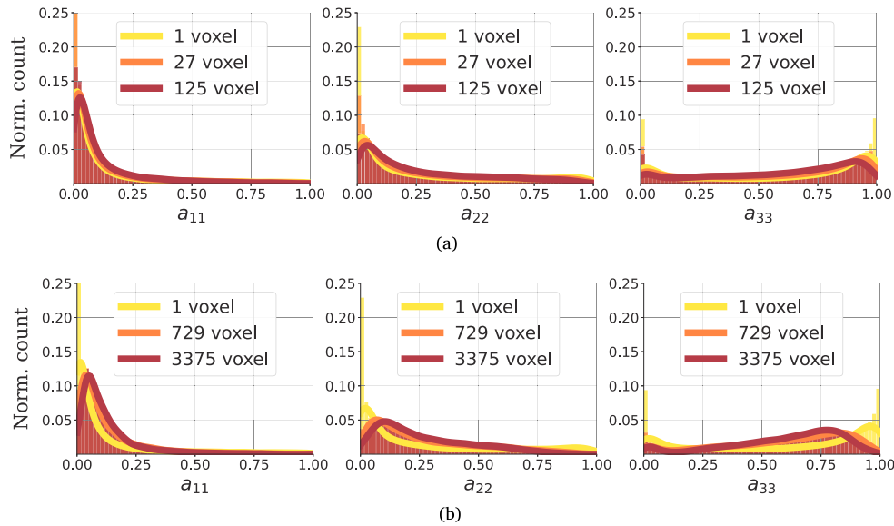
Fig. 14. Histograms of the three a_i components of the mapped second-order orientation tensor (according to Eq. (8)) for five different areas. The fibre orientation tensors are mapped onto 43,180 target integration points. The results for '1 voxel' (yellow curves) are computed based on one dominant fibre orientation vector p of the voxel, the target integration point lies in. (a) Three different areas where two (orange and red curve) homogenise fibre orientations of 27 and 125 voxels, respectively, around the target integration points. (b) Three different areas where two (orange and red curve) homogenise fibre orientations of 729 and 3375 voxels, respectively, around the target integration points. The solid lines represent Gaussian Kernel density estimations. (For interpretation of the references to colour in this figure legend, the reader is referred to the web version of this article.)
