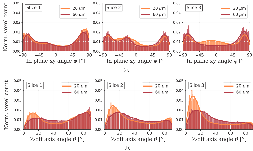
Fig. 6. Histograms of the in-plane xy (azimuthal) angle \varphi (a) and z-off (zenith) axis angle \theta (b) for the defined three slices in the Dome Scan and the two voxel-sizes 20 \mu\text{m} and 60 \mu\text{m} . The solid lines represent Gaussian Kernel density estimations. The voxel counts are normalised for better comparison.
