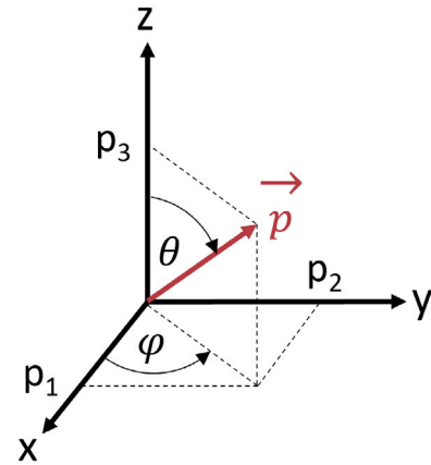
Fig. 3. The fibre orientation can be expressed as a unit vector (Eq. (3)) in Cartesian coordinates, where \varphi represents the in-plane angle between x -axis and the xy -projection of the unit vector, also denoted azimuth, and \theta the angle between the z -axis and the unit vector, also denoted zenith.
