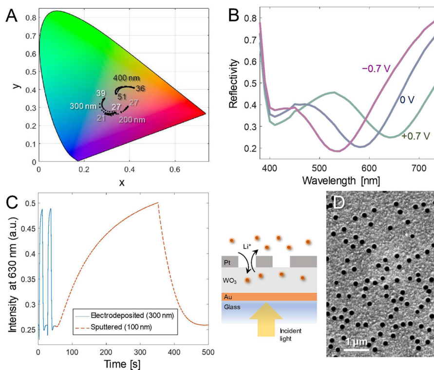
Figure 6. Electrochromic nanostructures with electrodeposited \text{WO}_3 between 20 nm Au and a Pt mirror. (A) Switching of samples visualized by the CIE diagram. Color changes for three different thicknesses are shown. The numbers are the brightness values ( Y ) measured at each end voltage. (B) Examples of spectra while switching a cavity with electrodeposited \text{WO}_3 (300 nm nominal thickness). Each line is pseudocolored on the basis of the measured spectrum. (C) Example of switching dynamics (intensity at 630 nm) in the PC electrolyte. The slower switch with sputtered \text{WO}_3 is included for comparison. Note that the electrodeposited film is thicker (but the nanostructures have a similar color). (D) Electron microscopy image of the Pt mirror with nanoholes (the backside of the structure) on top of electrodeposited \text{WO}_3 .
