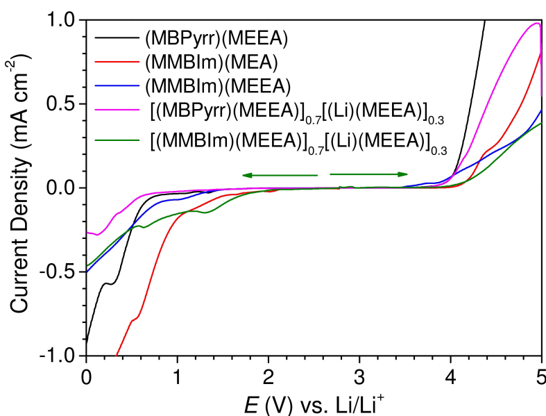
Figure 4. LSV curves of neat ILs and electrolytes on GC electrode at 20 °C.
