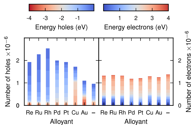
Figure 5. Number of hot carriers in the top surface for Ag-alloy NPs with a surface composition of 17% after excitation with a laser at the LSP peak (3.3 eV).
