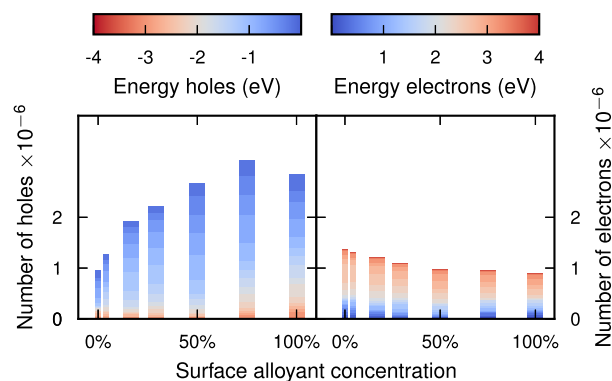
Figure 3. Number of HCs at the surface of the core–crown Ag–Pt NP for different surface alloy compositions by energetic range after excitation with a laser at the LSP peak (3.3 eV).
