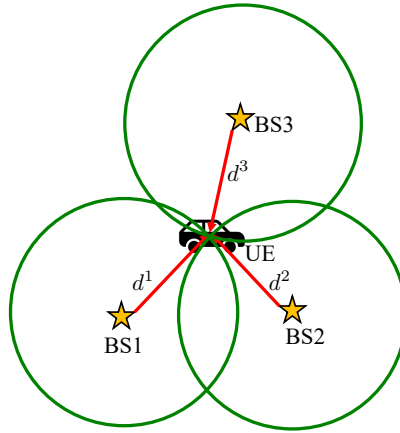
Figure 3.2: An example of ToA-based positioning method in a 2D scenario involving three BSs.
