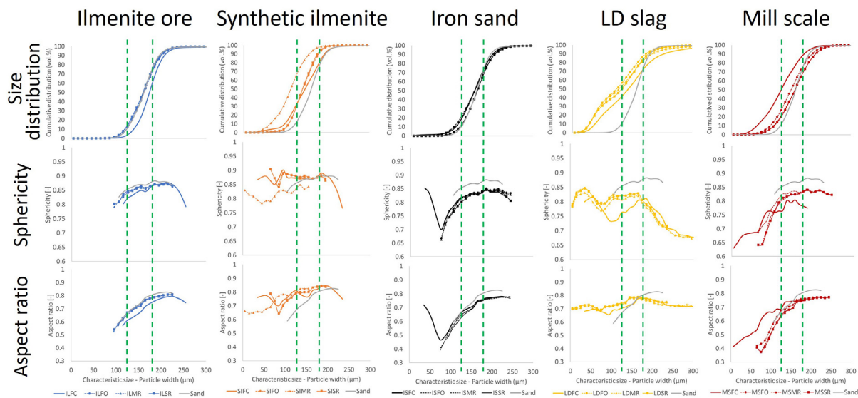
Fig. 7. Measured sphericity and aspect ratio of all oxygen carrier samples and sand plotted against characteristic size. The green dashed lines indicate the original sieving size range (125–180 μm).
