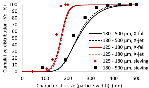
Fig. 3. Comparison between X-fall and X-jet dispersion methods for particle size analysis of ILFC.
