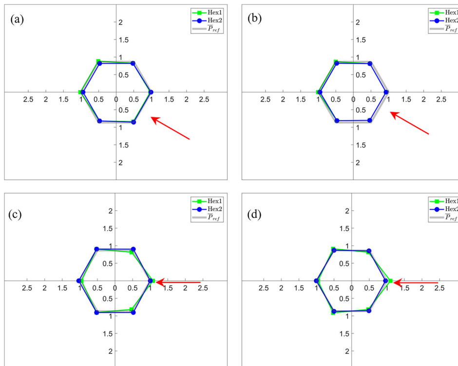
Figure 10. Normalised power generated from each WEC unit in the Hex1-120 and Hex2 layouts under EC3 with the incident wave direction of 150^\circ for (a) WaveEL 3.0 and (b) WaveEL 4.0, and 180^\circ for (c) WaveEL 3.0 and (d) WaveEL 4.0. Note that the polar coordinate system is used here, and the unit positions correspond to Figure 3(a). The red arrows indicate the incident wave directions.
