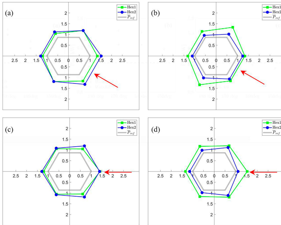
Figure 9. Normalised power generated from each WEC unit in the Hex1-120 and Hex2 layouts under EC2 with the incident wave direction of 150^\circ for (a) WaveEL 3.0 and (b) WaveEL 4.0, and 180^\circ for (c) WaveEL 3.0 and (d) WaveEL 4.0. Note that the polar coordinate system is used here, and the unit positions correspond to Figure 3(a). The red arrows indicate the incident wave directions.
